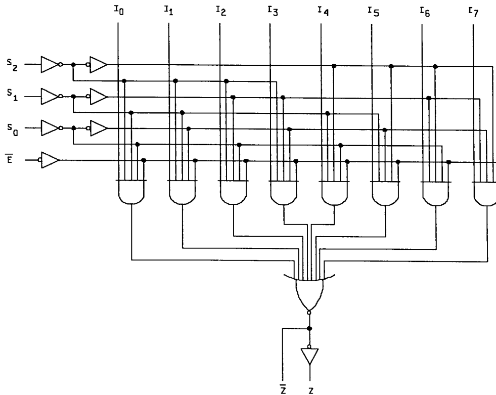
Figure 3. Logic diagram.
