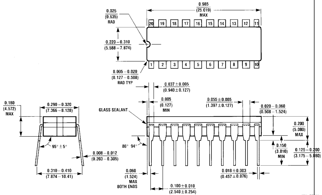
20-Lead Ceramic Dual-in-line J20A
