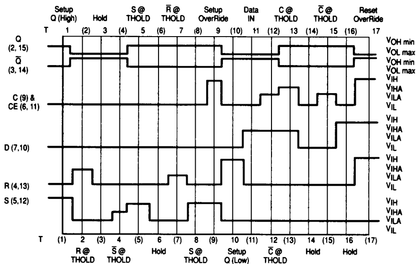
Figure 3. Timing Diagram
