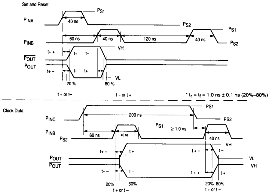
Figure 1. Switching Test Circuit and Waveforms
