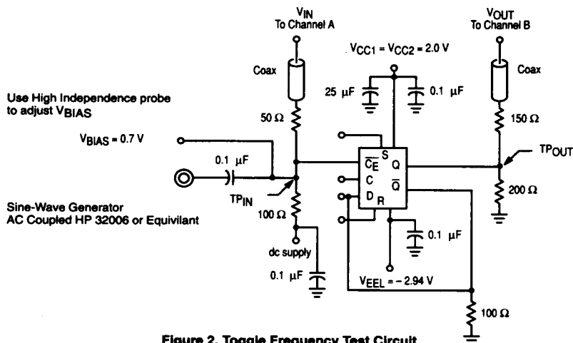
Figure 2. Toggle Frequency Test Circuit
