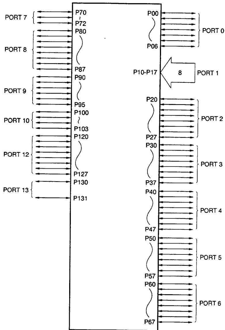
Figure 7-1. Port Configuration
