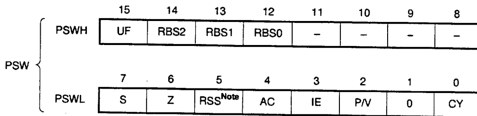
Figure 6-6. Program Status Word (PSW) Format
