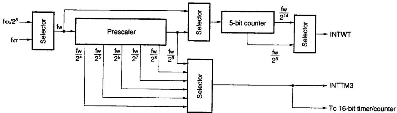
Figure 7-16. Block Diagram of Watch Timer
