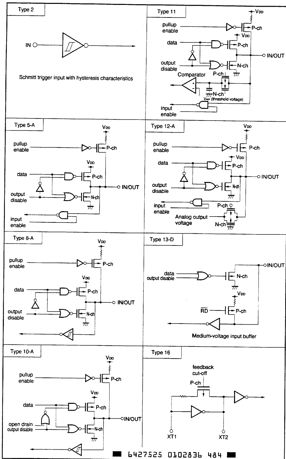
Figure 5-1. Types of Pin I/O Circuits
