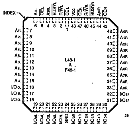
48-PIN LCC/FLATPACK TOP VIEW 2692 drw 03
