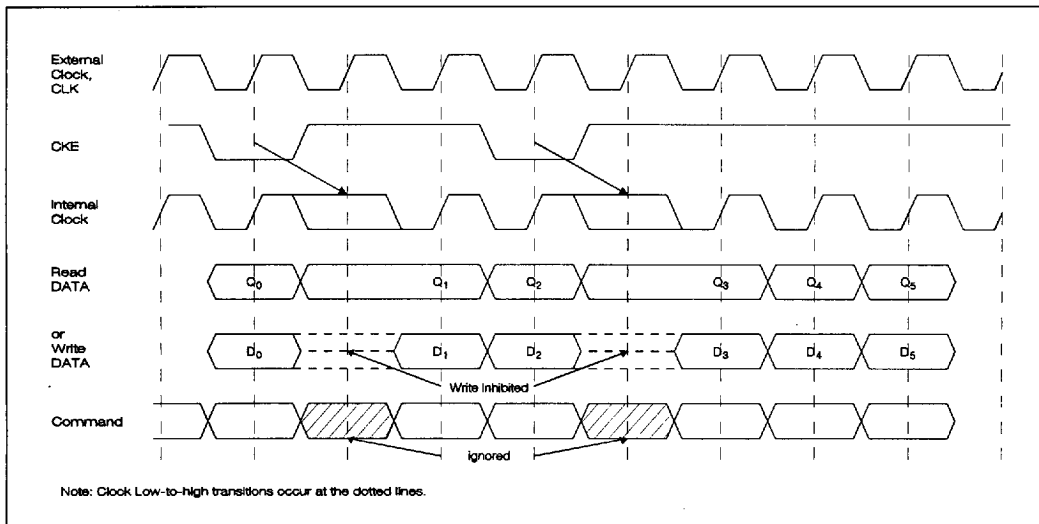
Figure 16. Example timing and control for Clock Suspend Operation
