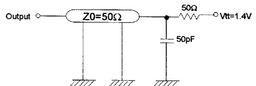
AC Output Load Circuit
