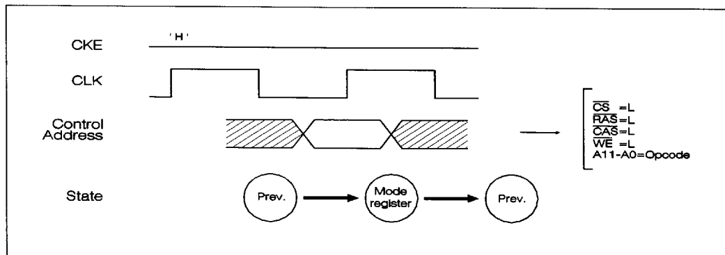
Figure 2. Timing of mode register set (program latency and burst).
