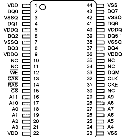
2Mx8 Synchronous DRAM 400mil x 725mil 44pin TSOP-II
