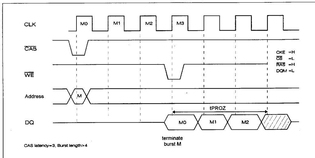
Figure 8. Timing of burst terminate command with read burst in progress.
