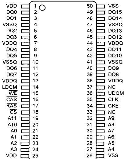
1Mx16 Synchronous DRAM 400mil x 825mil 50pin TSOP-II
