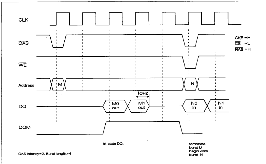
Figure 7. Timing of write initiation with read burst in progress.
