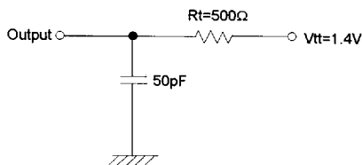
DC Output Load Circuit
