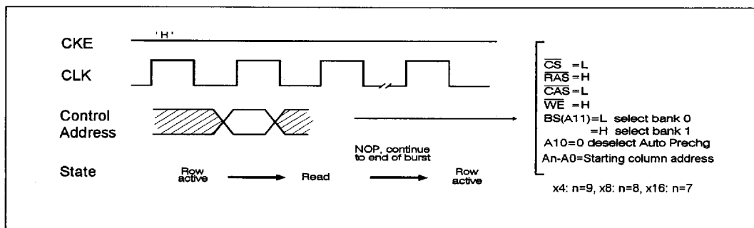
Figure 5. Burst read sequence, Auto Precharge Deselected.
