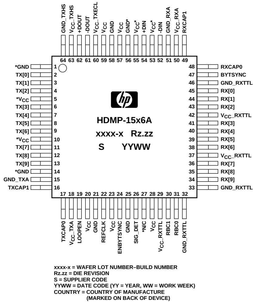
Figure 11. HDMP-1536/46A (TRx) Package Layout and Marking, Top View.
