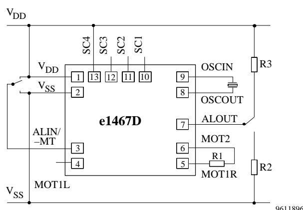
Figure 5. Functional test
