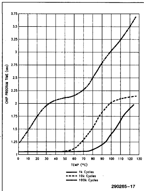
Figure 7. 28F512 Typical Program Time at 12V See Note 1, Page 2-56.
