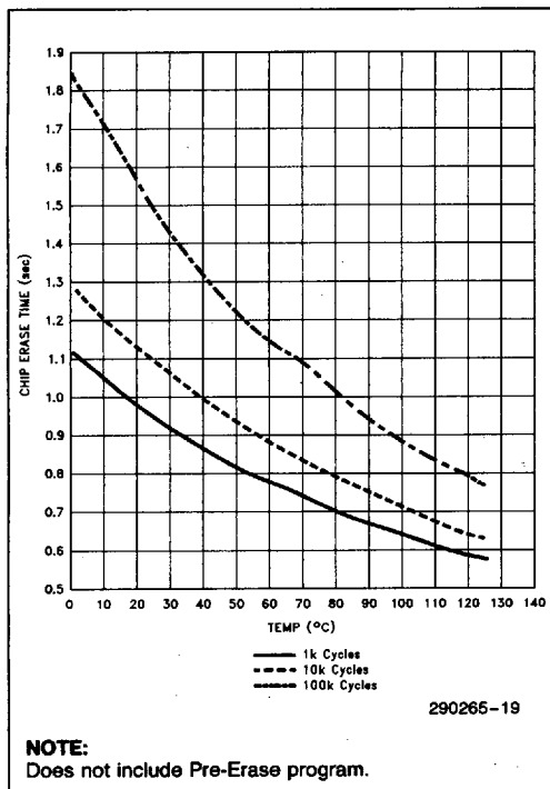
Figure 9. 28F512 Typical Erase Time at 12V See Note 1, Page 2-56.
