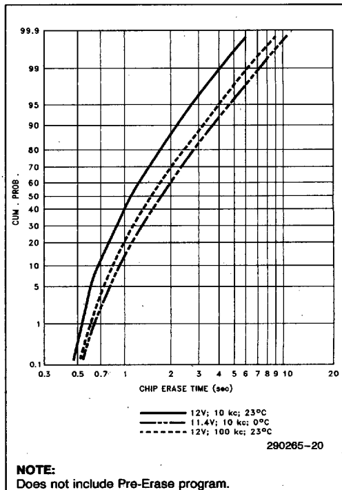
Figure 10. 28F512 Typical Erase Capability
