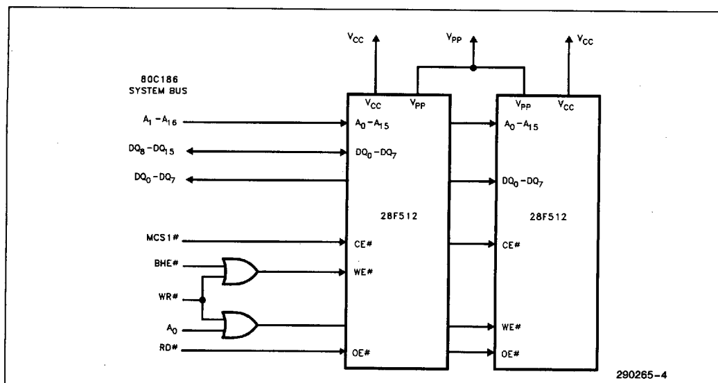
Figure 3. 28F512 in an 80C186 System
