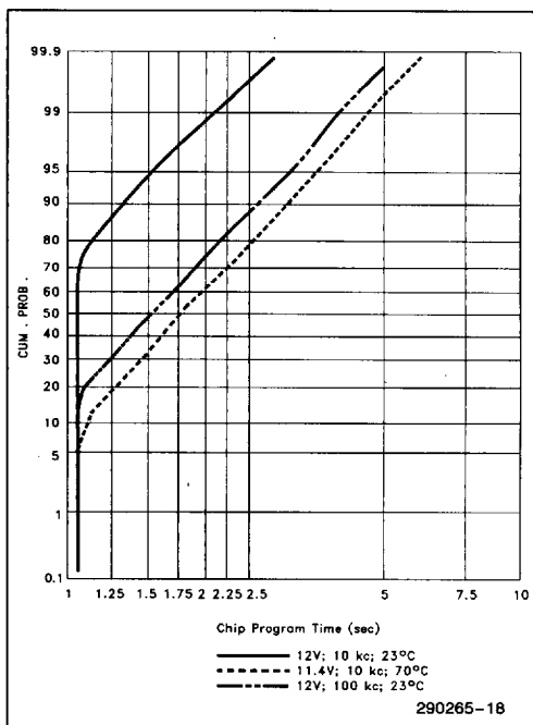
Figure 8. 28F512 Typical Programming Capability
