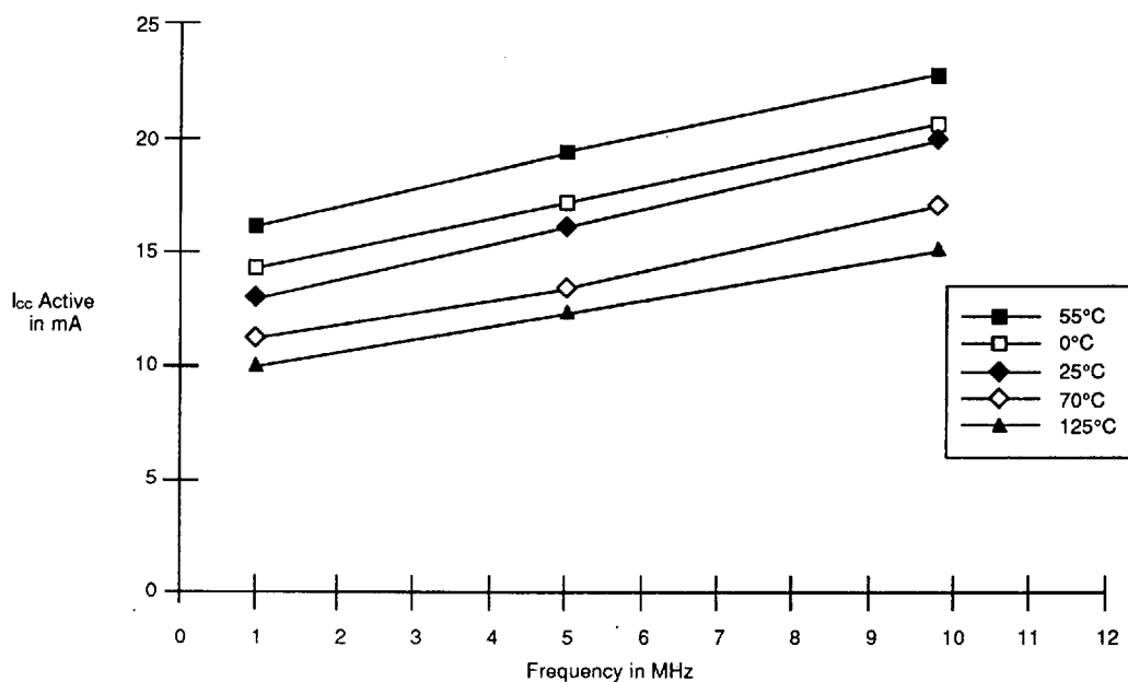
Figure 5. Am28F512—Average I_{cc} Active vs. Frequency
