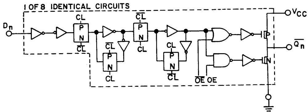
FIGURE 3. Logic diagram.
