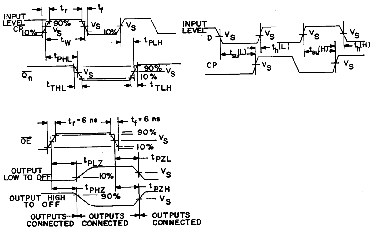
FIGURE 4. Switching waveforms.
