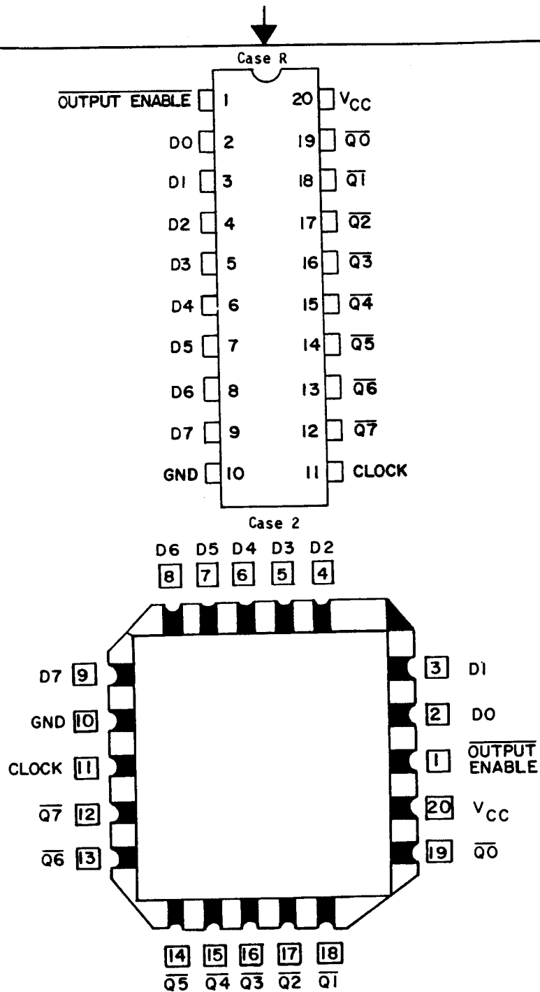
FIGURE 1. Terminal connections.
