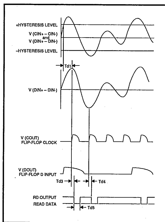
FIGURE 2: Timing Diagram
