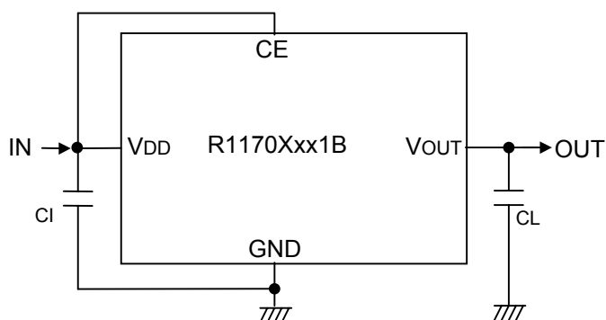
Example of the typical application of R1170XxxxB
