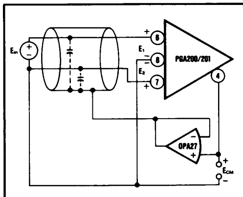
FIGURE 4. Guard Drive.
