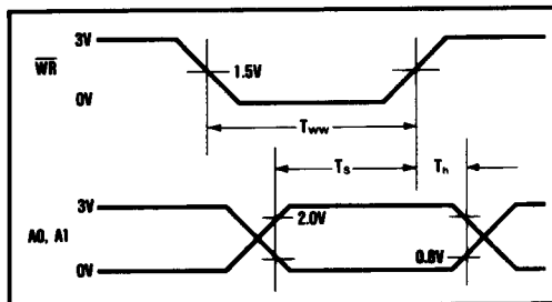
FIGURE 2. Timing Diagrams.
