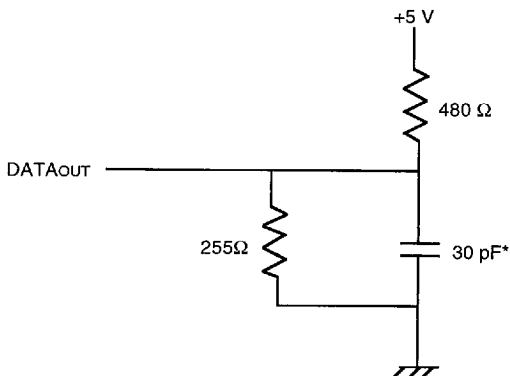
Figure 1. Output Load
