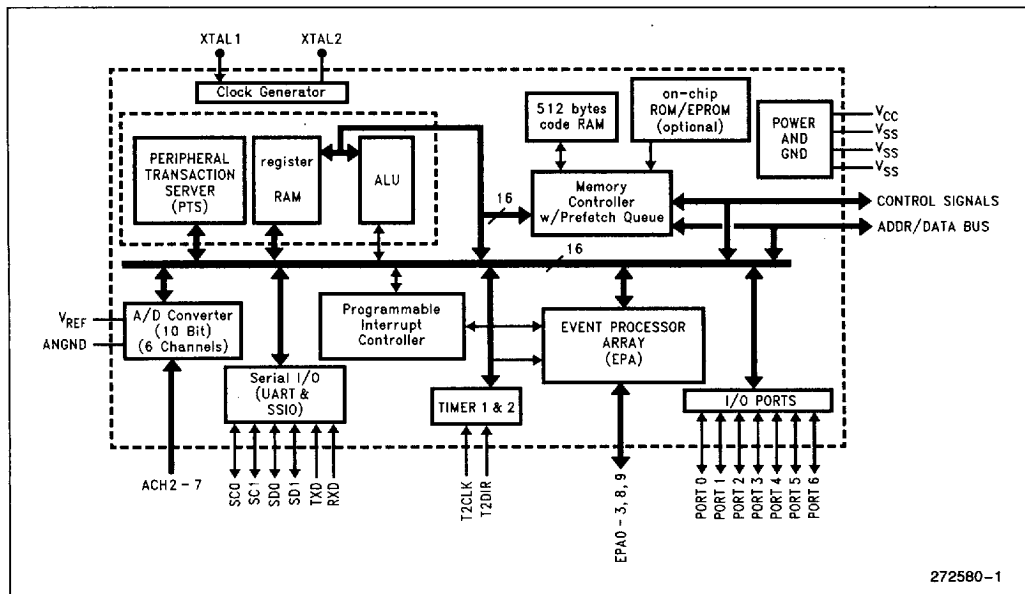
Figure 1. Block Diagram
