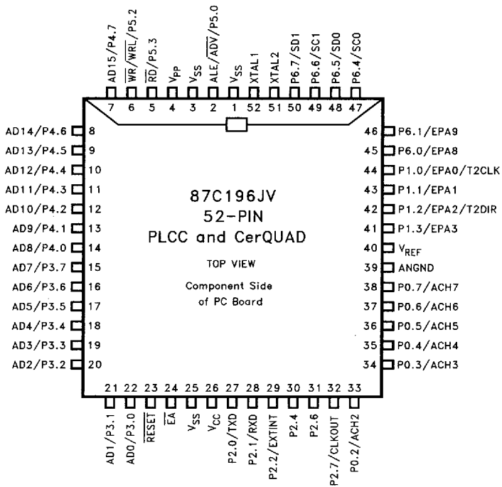
Figure 3. Package Diagram
