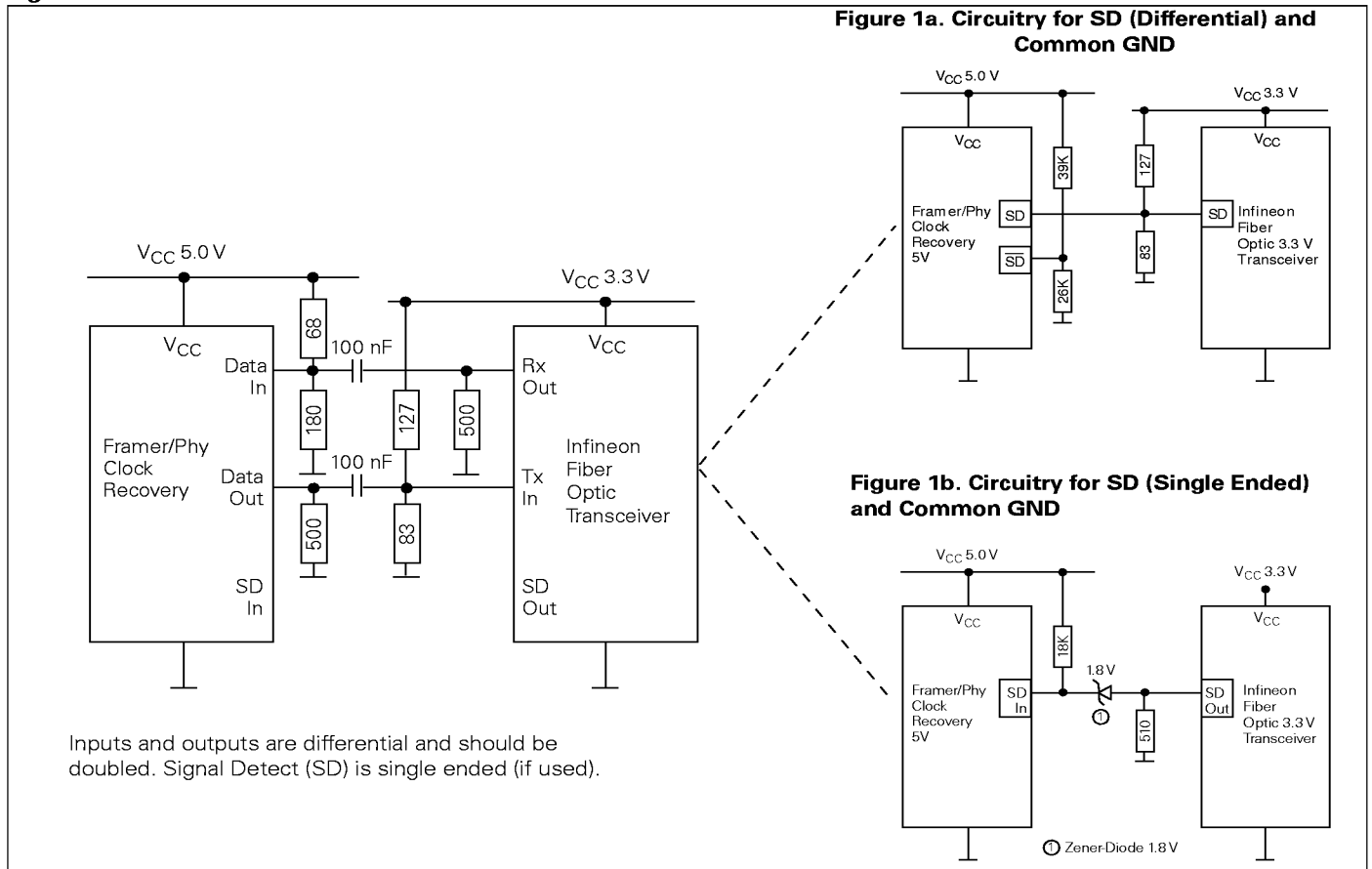
Figure 1. Common GND
