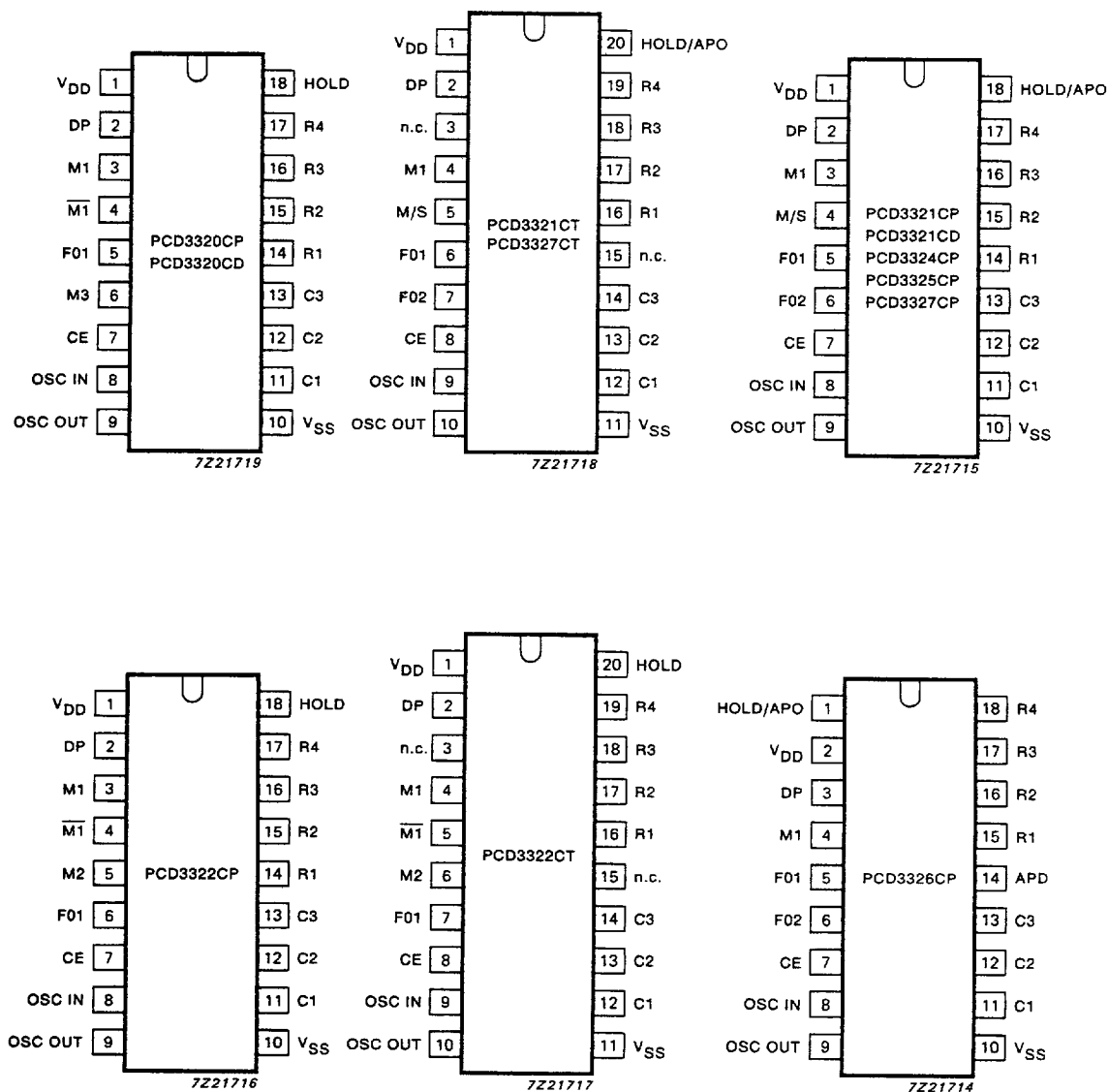
Fig.2 Pinning diagrams.
