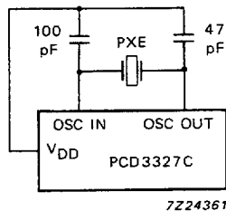
Fig.18 PCF3327 oscillator circuit.
