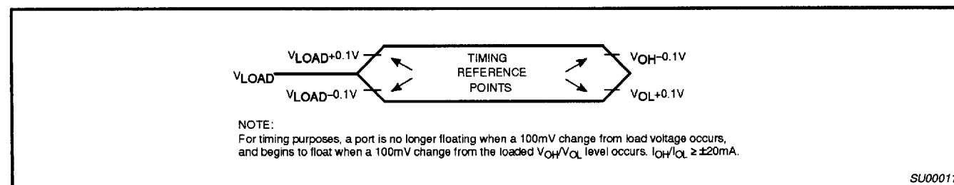
Figure 25. Float Waveform
