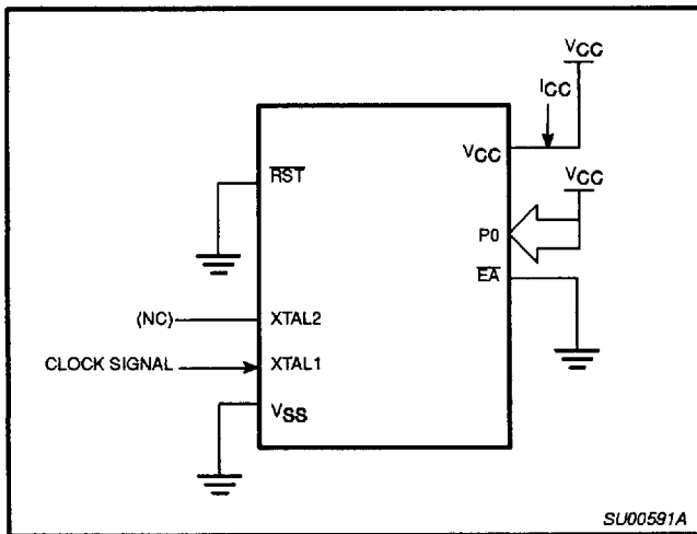
Figure 26. I_{CC} Test Condition, Active Mode All other pins are disconnected
