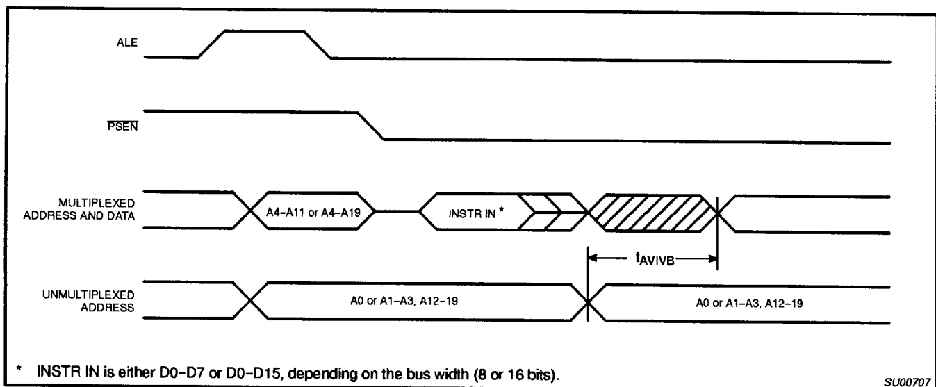
Figure 17. External Program Memory Read Cycle (Non-ALE Cycle)
