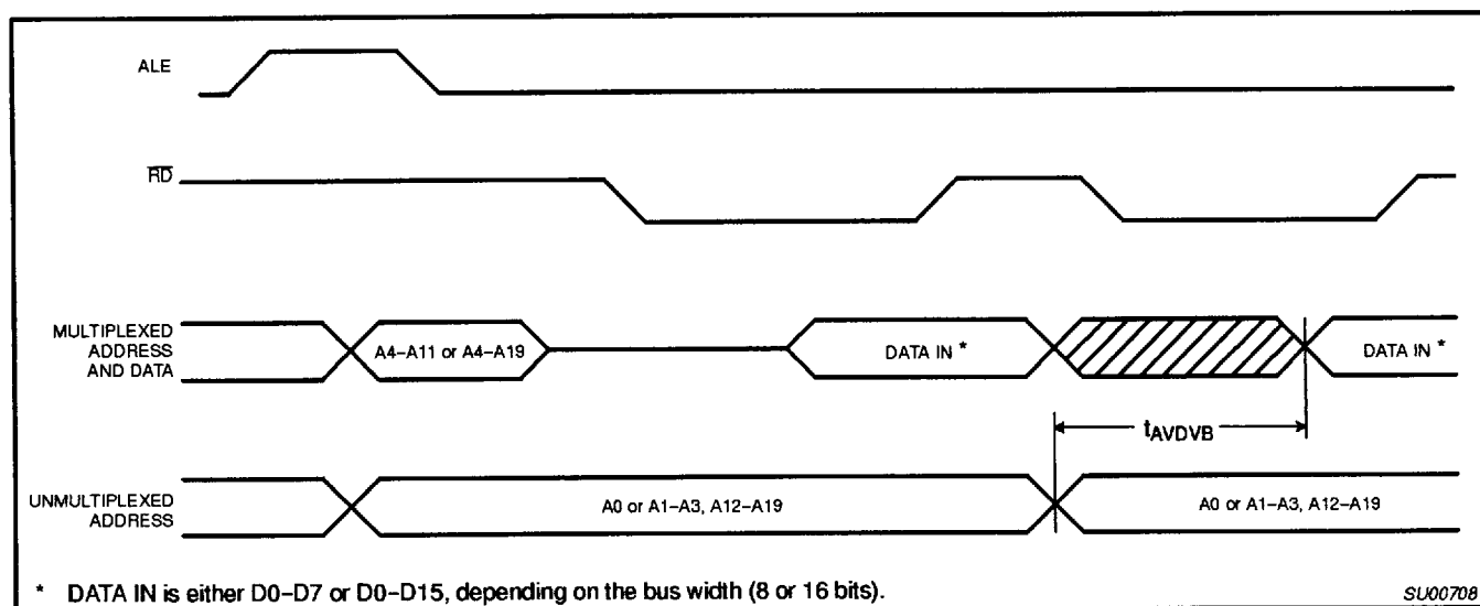
Figure 19. External Data Memory Read Cycle (Non-ALE Cycle)
