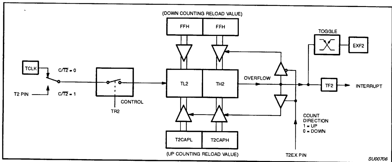
Figure 9. Timer 2 Auto Reload Mode (DCEN = 1)
