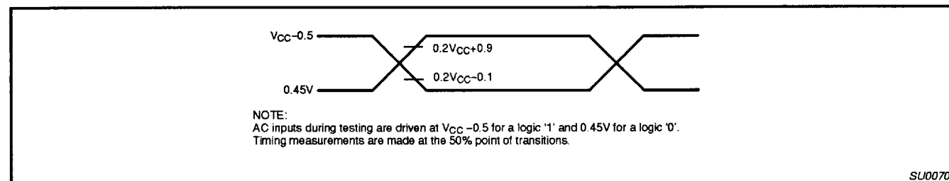
Figure 24. AC Testing Input/Output
