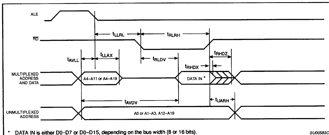
Figure 18. External Data Memory Read Cycle (ALE Cycle)
