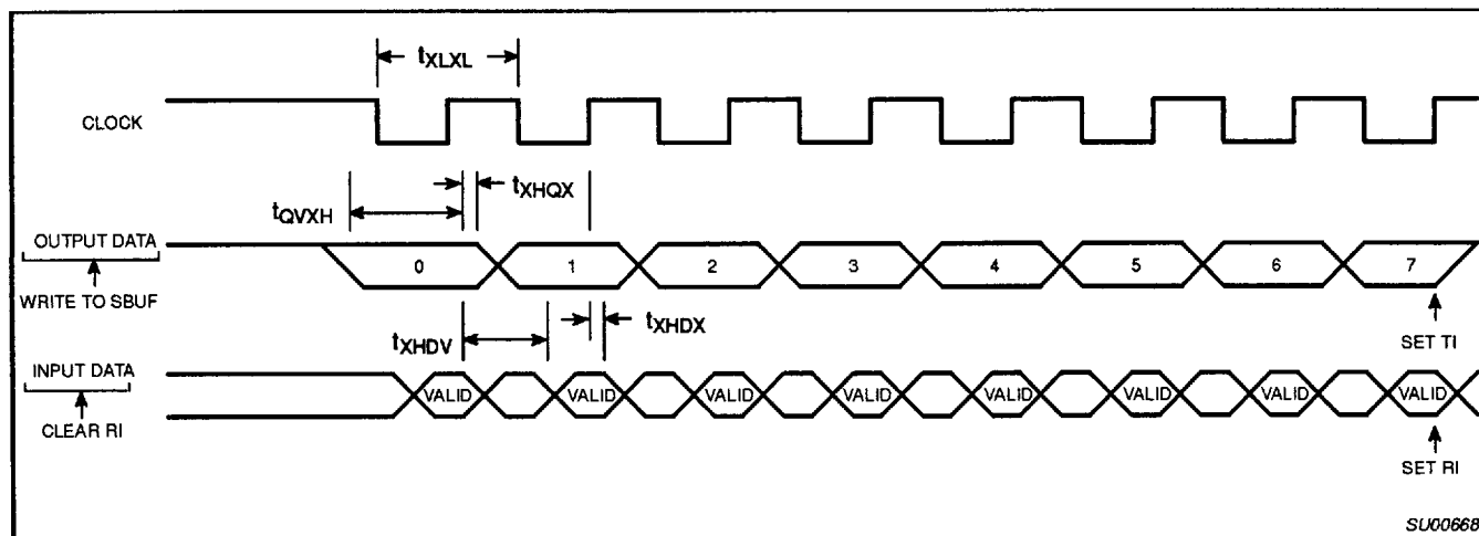
Figure 22. Shift Register Mode Timing
