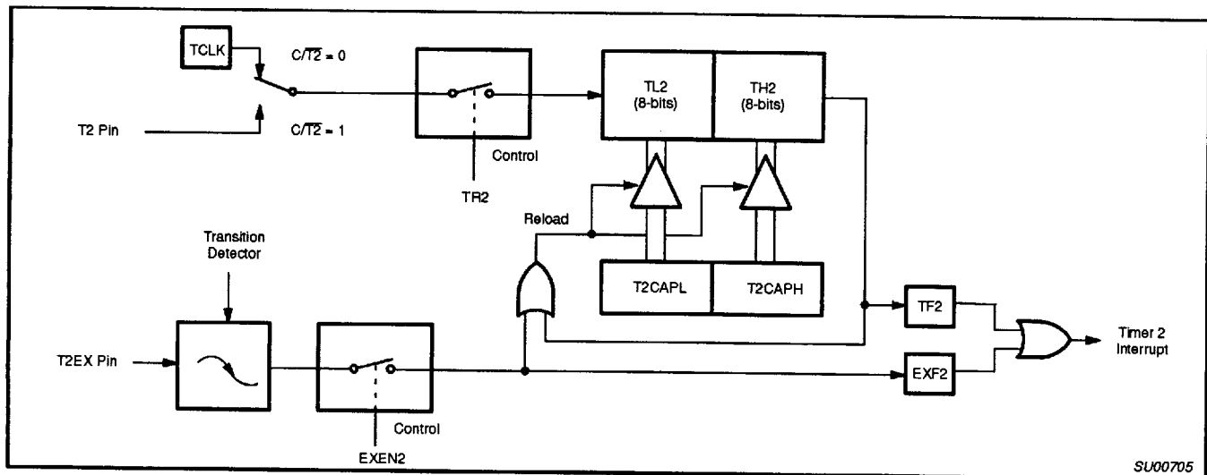
Figure 8. Timer 2 in Auto-Reload Mode (DCEN = 0)
