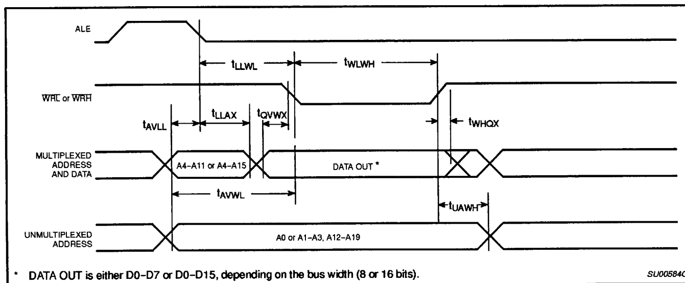
Figure 20. External Data Memory Write Cycle
