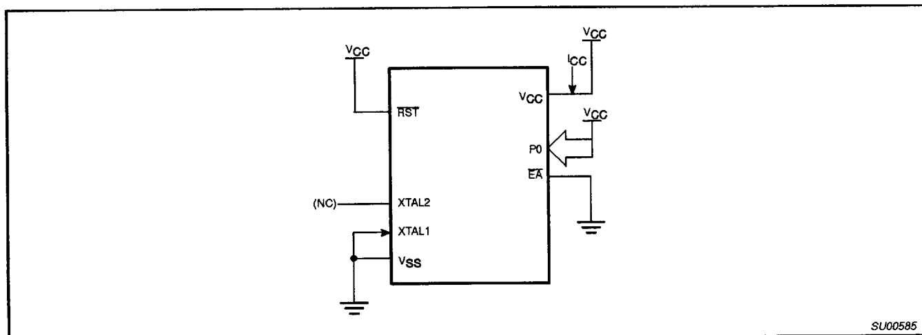
Figure 30. I_{CC} Test Condition, Power Down Mode All other pins are disconnected. V_{CC}=2V to 5.5V
