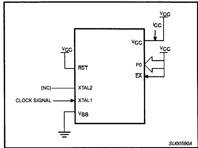
Figure 27. I_{CC} Test Condition, Idle Mode All other pins are disconnected
