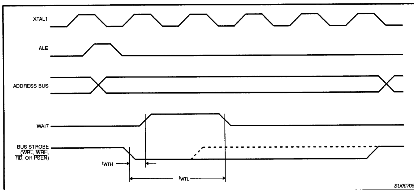
Figure 21. WAIT Signal Timing
