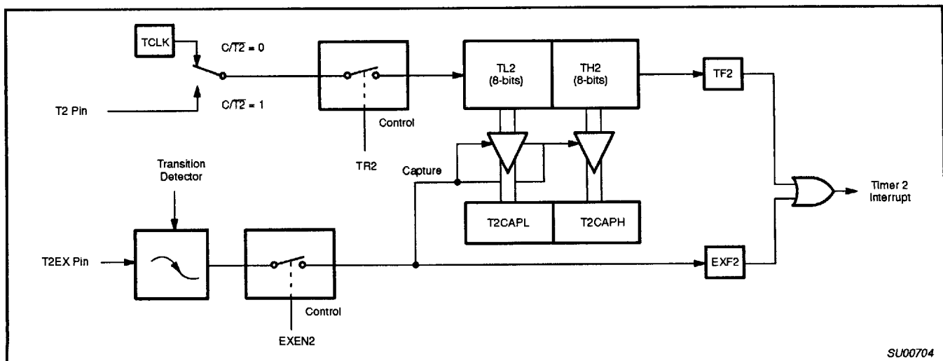
Figure 7. Timer 2 In Capture Mode
