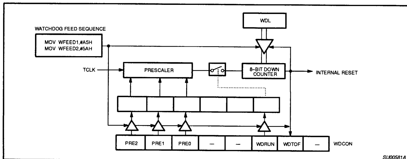
Figure 10. Watchdog Timer in XA-G3
