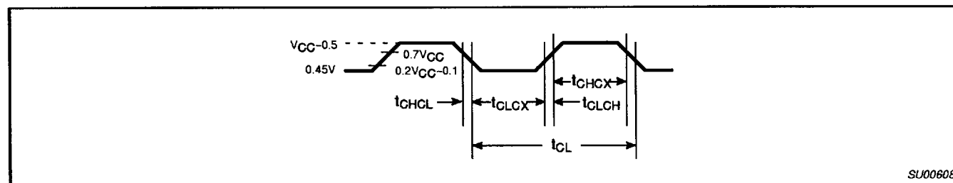
Figure 23. External Clock Drive
