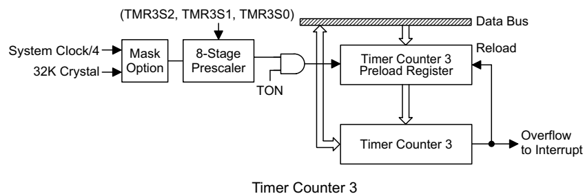
TMR3 register
