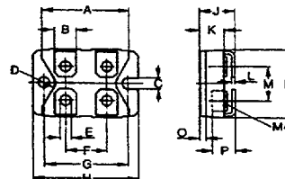
MINIBLOC SOT-227 B M4 screws (4x) supplied
