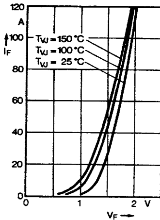
Fig. 1 Forward current versus voltage drop
