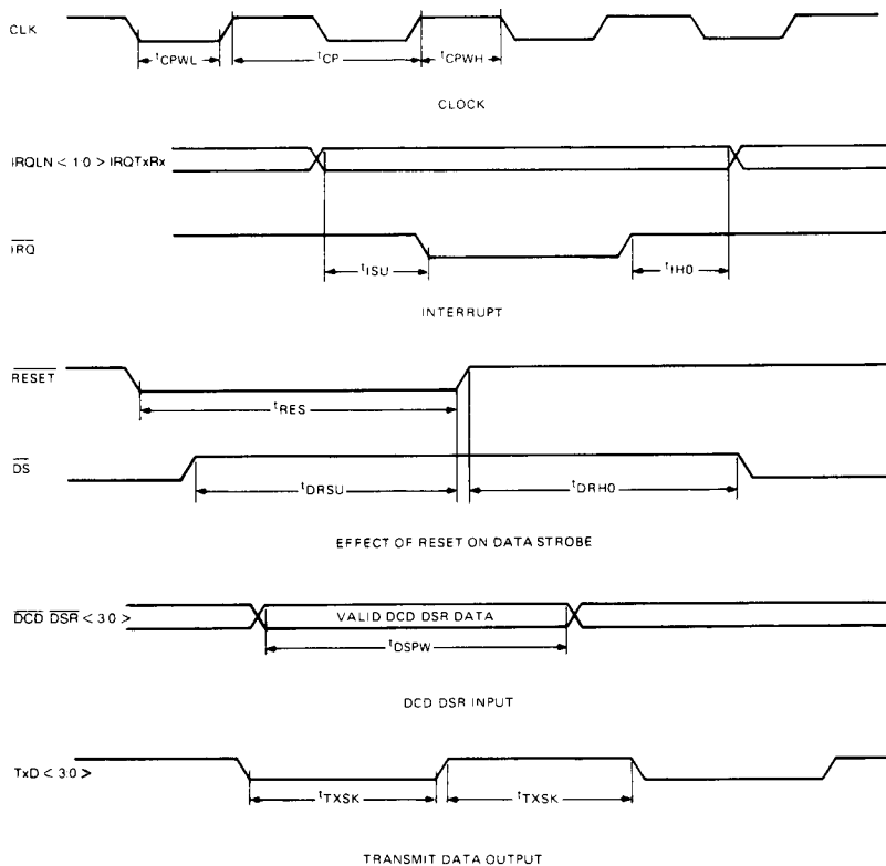
FIGURE 12—COM78C804 MISCELLANEOUS SIGNAL TIMING
