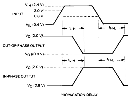
FIGURE 13—COM78C804 PROPAGATION DELAY AND SETUP AND HOLD VOLTAGE WAVEFORMS
