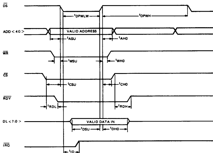
FIGURE 11—COM78C804 BUS WRITE CYCLE TIMING
