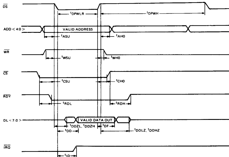
FIGURE 10—COM78C804 BUS READ CYCLE TIMING
