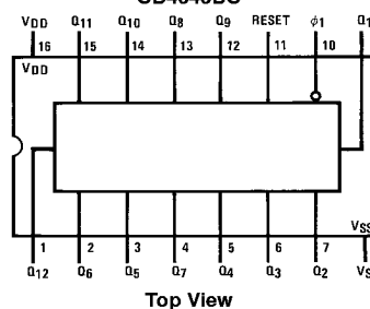
Pin Assignments for DIP, SOIC and SOP CD4040BC
