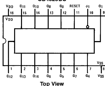
Pin Assignments for DIP and SOIC CD4020BC
