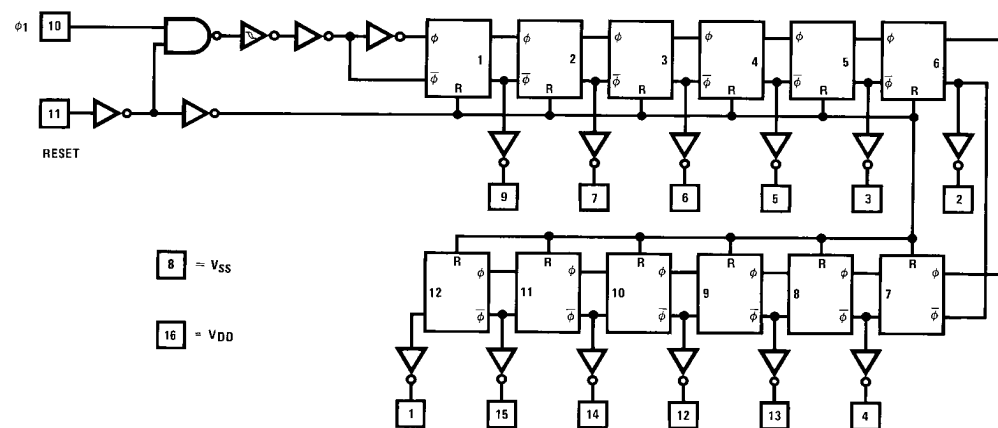
CD4040BC
