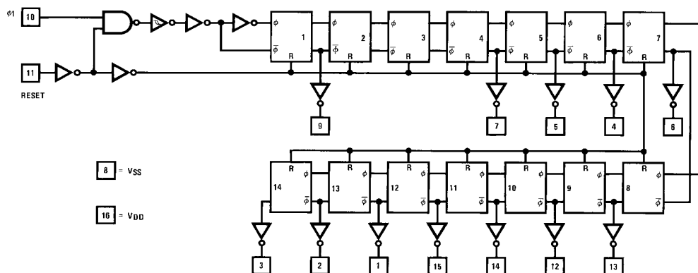
CD4020BC
