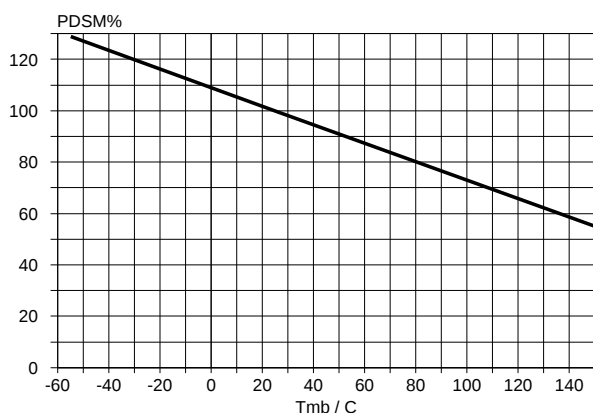
Fig.10. Normalised limiting overload dissipation. P_{DSM\%} = 100 \cdot P_{DSM}/P_{DSM(25^\circ C)} = f(T_{mb})
