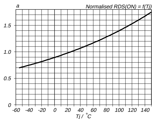
Fig.8. Normalised drain-source on-state resistance. a = R_{DS(ON)}/R_{DS(ON)25^\circ C} = f(T_J) ; I_D = 7.5\text{ A} ; V_{IS} = 5\text{ V}
