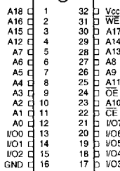
DIP Top View
