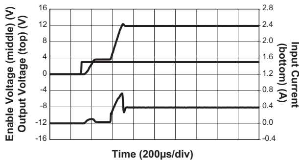
AAT1230 Soft Start (V_{IN} = 3.6V; C_{IN} = 2.2\mu F; I_{OUT} = 100mA; V_{OUT} = 12V)
