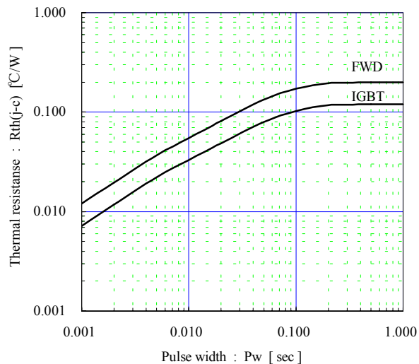
a Transient thermal resistance (max.)
