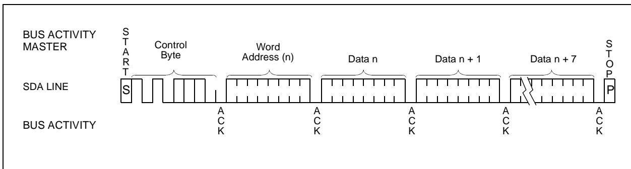
FIGURE 4-2: PAGE WRITE
