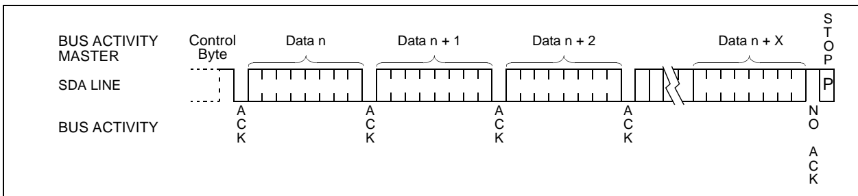
FIGURE 6-3: SEQUENTIAL READ
