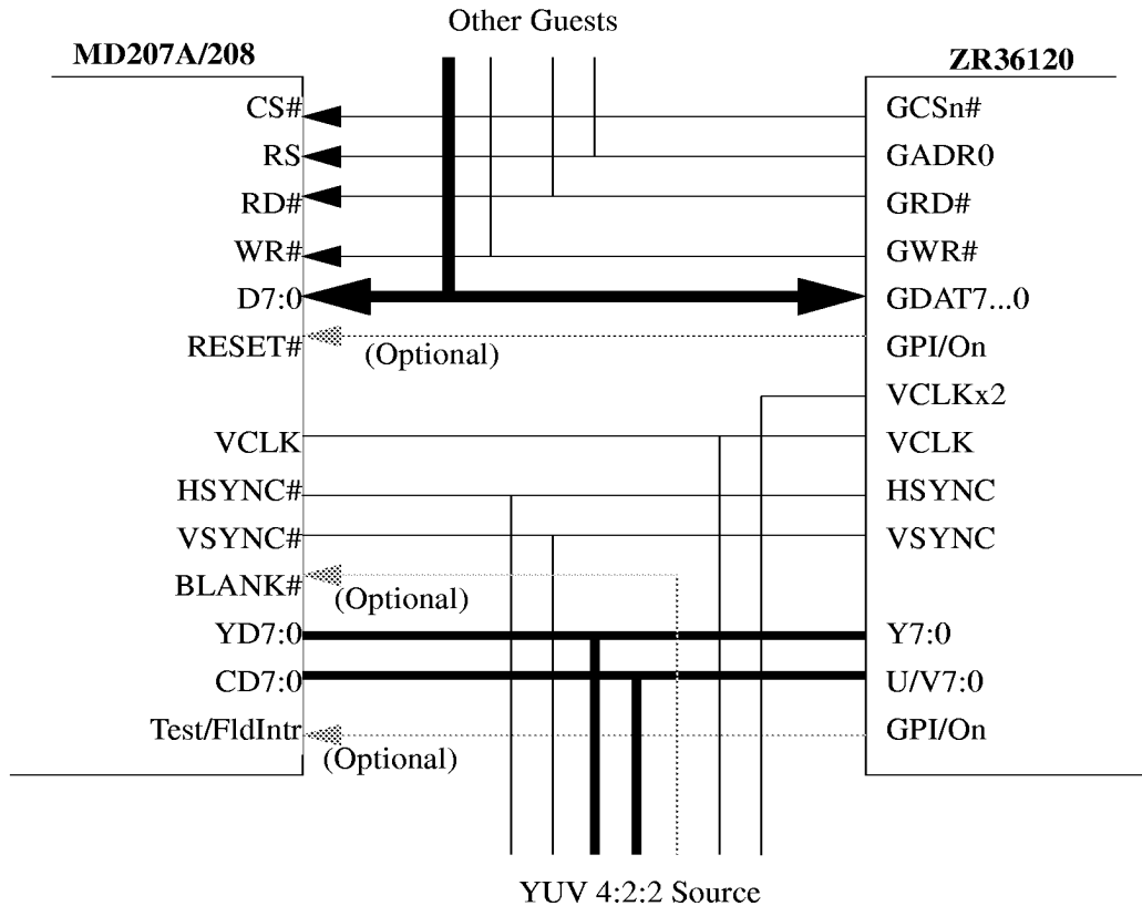
Figure 9: ZR36120 - MD207A/208 Basic Interconnection
