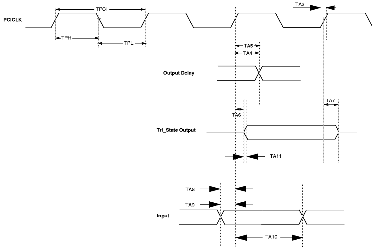
Figure 4: PCI Bus Interface Timing
