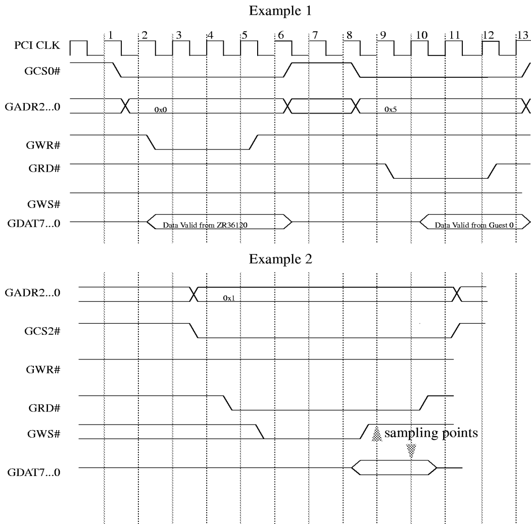
Figure 3: Two examples of GuestBus cycles
