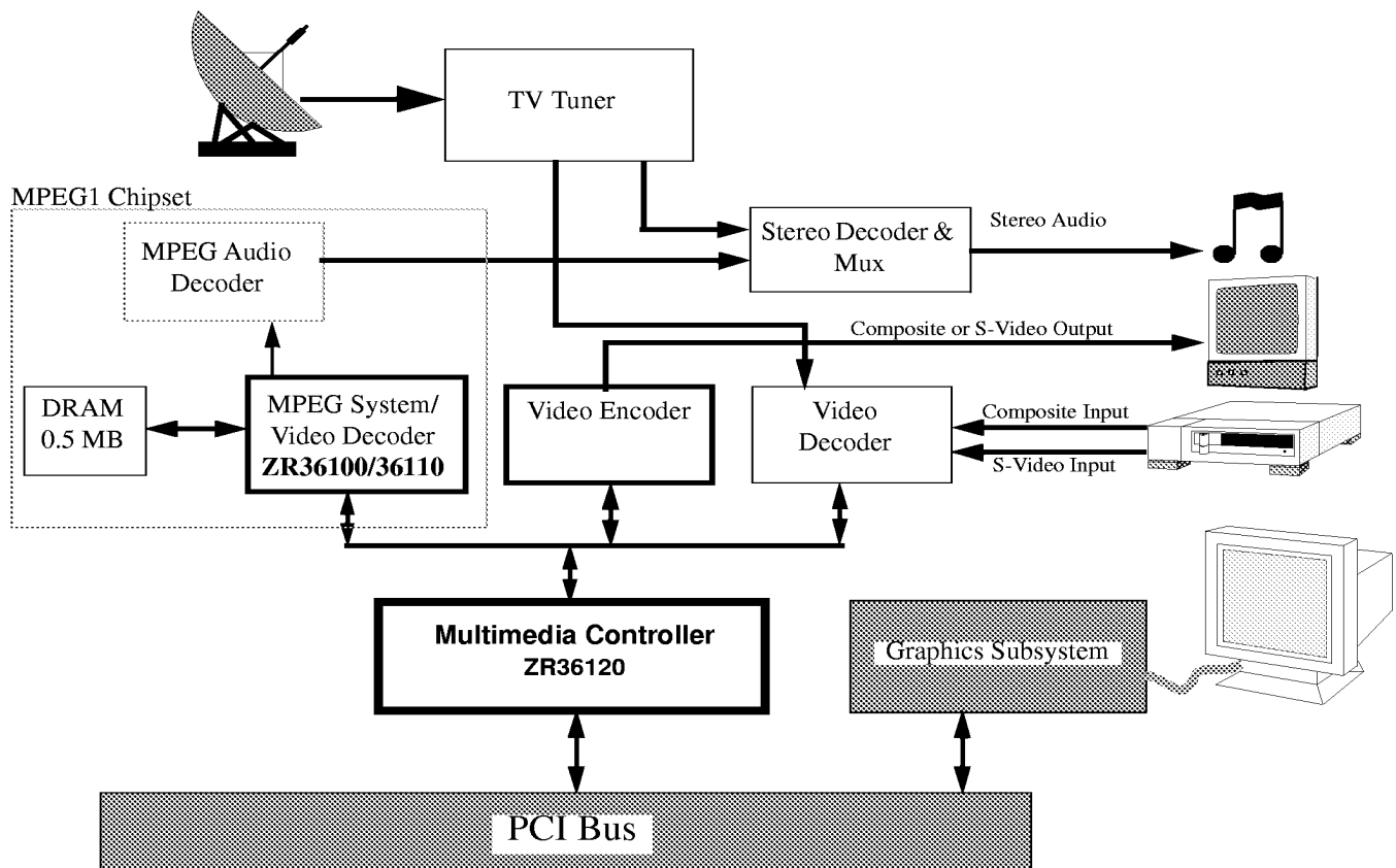
Figure 1: Block Diagram of A Typical Video Subsystem for PCI Computers
