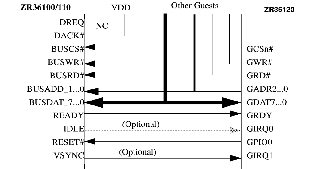
Figure 8: ZR36120 - ZR36100/ZR36110 Host (Guest) Bus Interconnection
