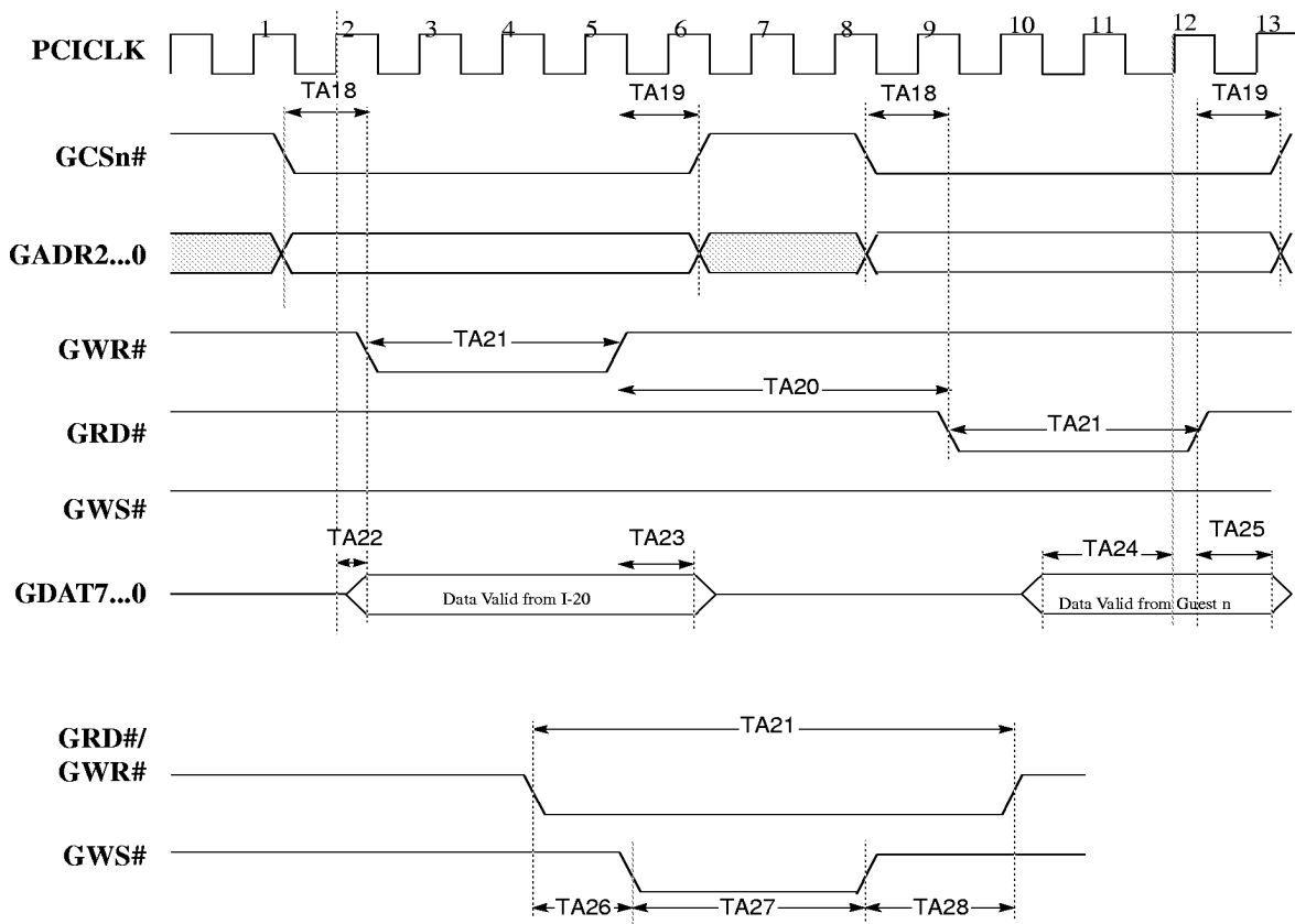
Figure 6: GuestBus Timing
