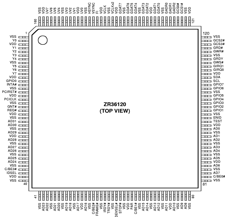
Figure 7: 160-Pin Quad Flat Pack Pinout
