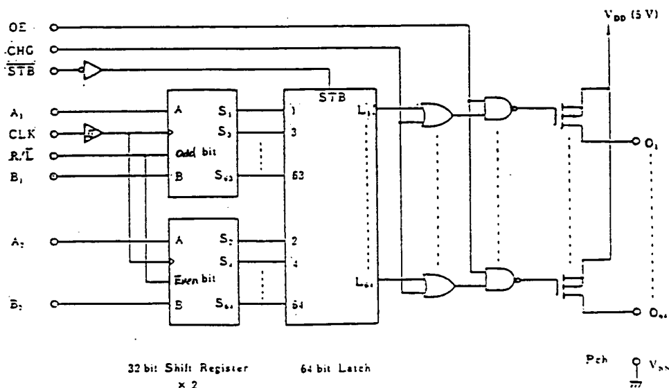
(BLOCK DIAGRAM)
