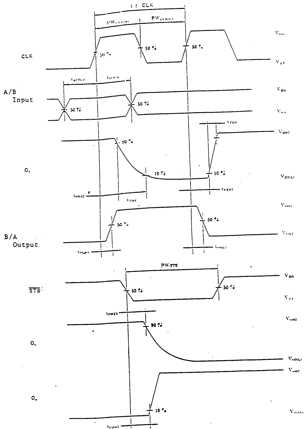
(AC Characteristics Wave Chart)
