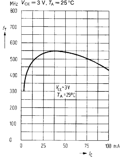
Transition frequency versus collector current
