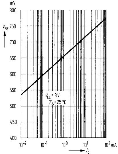
Base-emitter voltage versus input current
