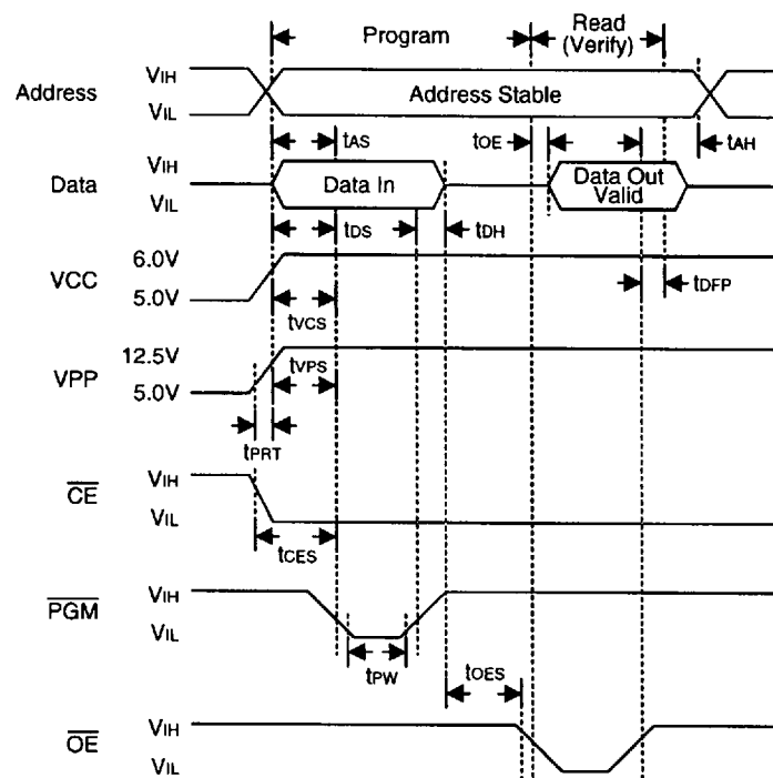
Figure 2. Programming waveforms
