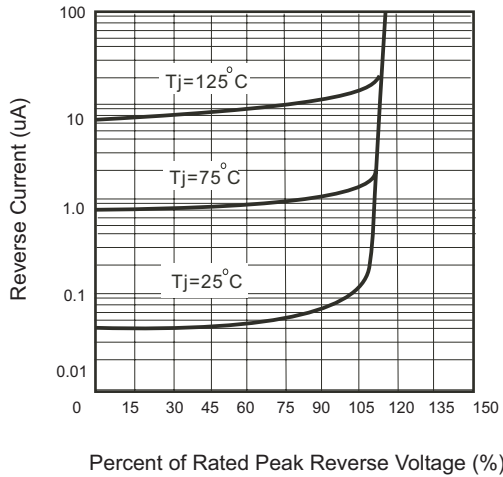
Fig. 1 - Reverse Characteristics
