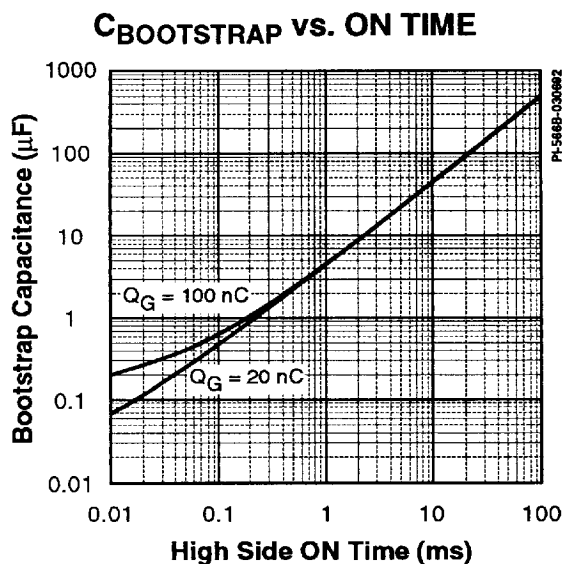
Figure 6. High-side On Time versus Bootstrap Capacitor.
