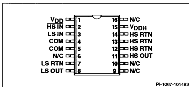
Figure 2. Pin Configuration.
