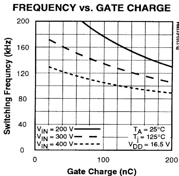
Figure 5. Gate Charge versus Switching Frequency.
