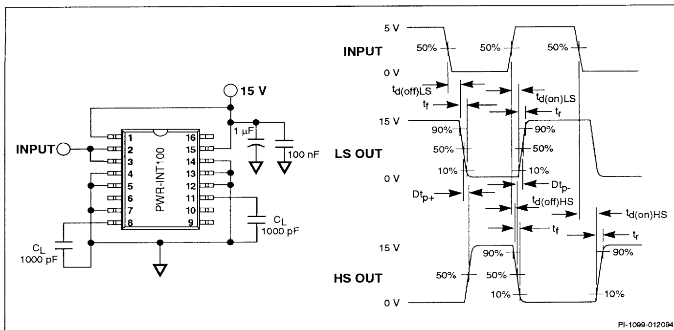
Figure 7. Switching Time/Deadtime Test Circuit.
