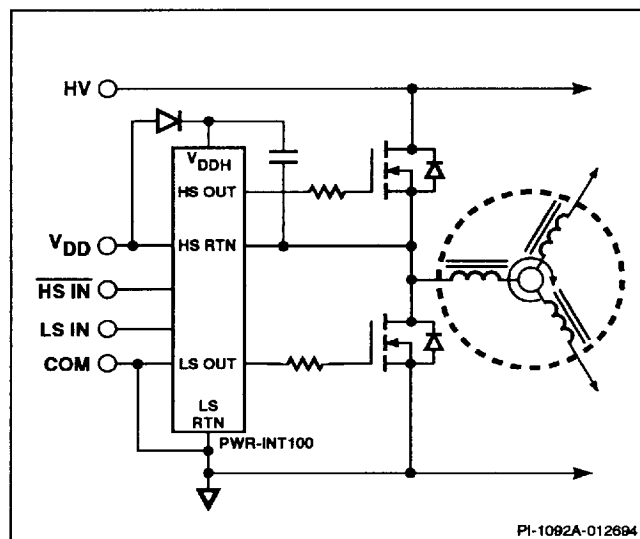
Figure 1. Typical Application
