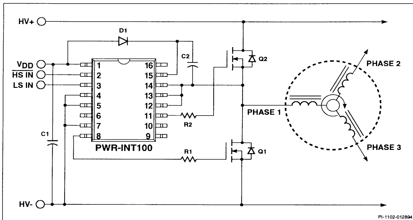
Figure 4. Using the PWR-INT100 in a 3-phase Configuration.
