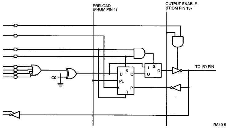
Figure 1. PLDC20RA10 Macrocell
