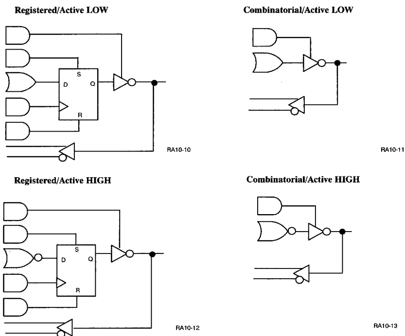
Figure 3. Four Possible Macrocell Configurations for the PLDC20RA10
