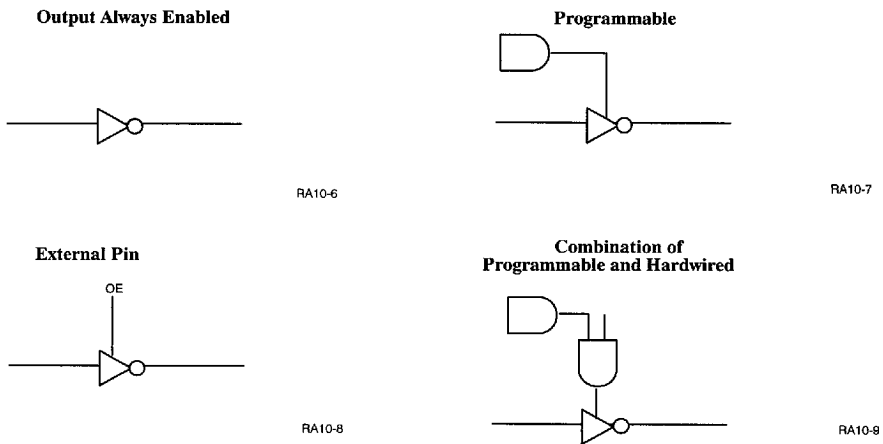
Figure 2. Four Possible Output Enable Alternatives for the PLDC20RA10
