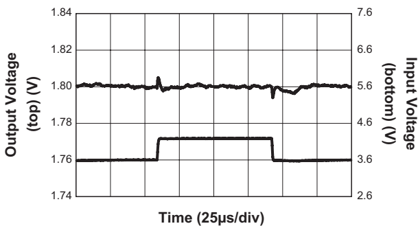
Step-Down Converter Line Transient ( V_{OUT} = 1.8V @ 400mA )
