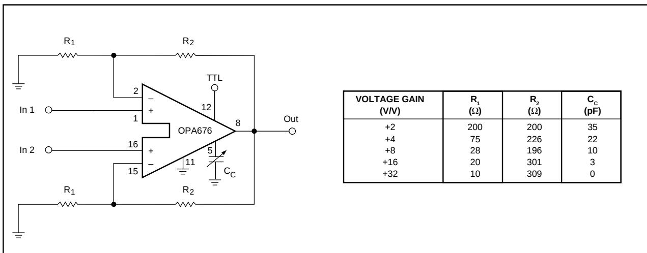
FIGURE 20. Two-Input Multiplexer (with gain).
