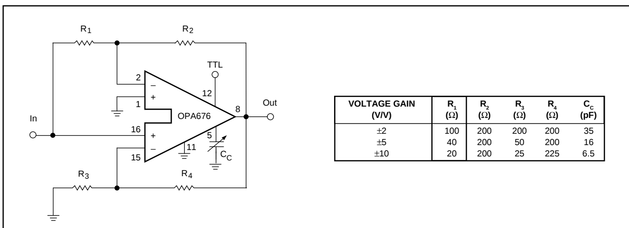
FIGURE 21. Synchronous Modulator/Demodulator (with gain).
