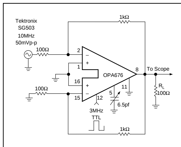
FIGURE 5. OPA676 Input Selection Transition Time Test Circuit.
