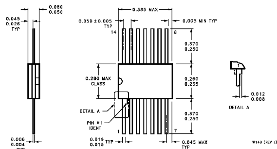
14-Lead Ceramic Flat Package (W) Order Number 5486FMBQ or DM5486W NS Package Number W14B
