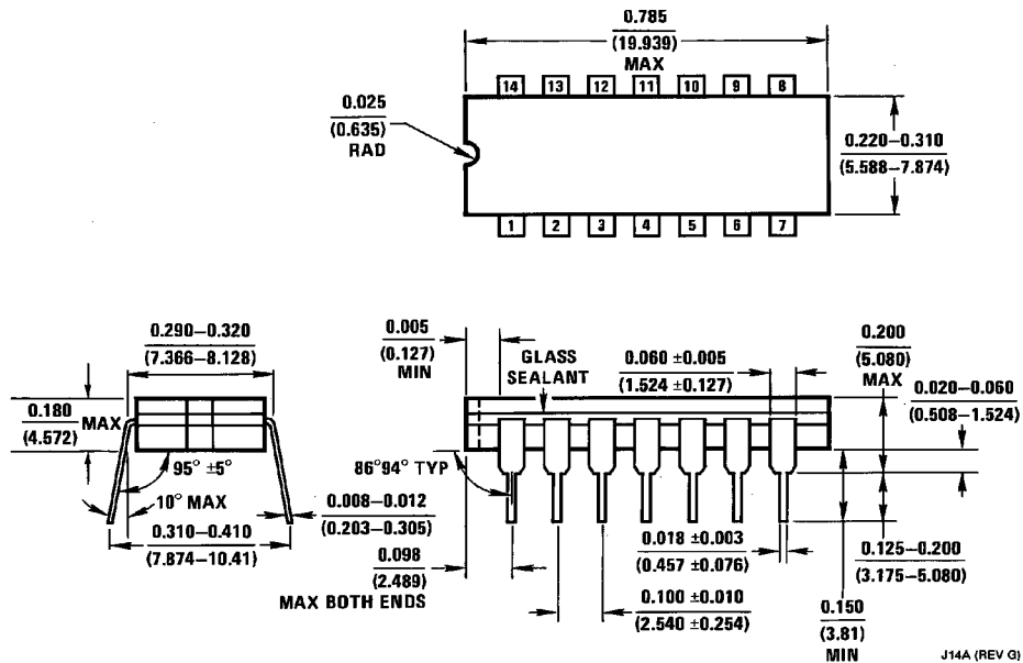
14-Lead Ceramic Dual-In-Line Package (J) Order Number 5486DMQB or DM5486J NS Package Number J14A
