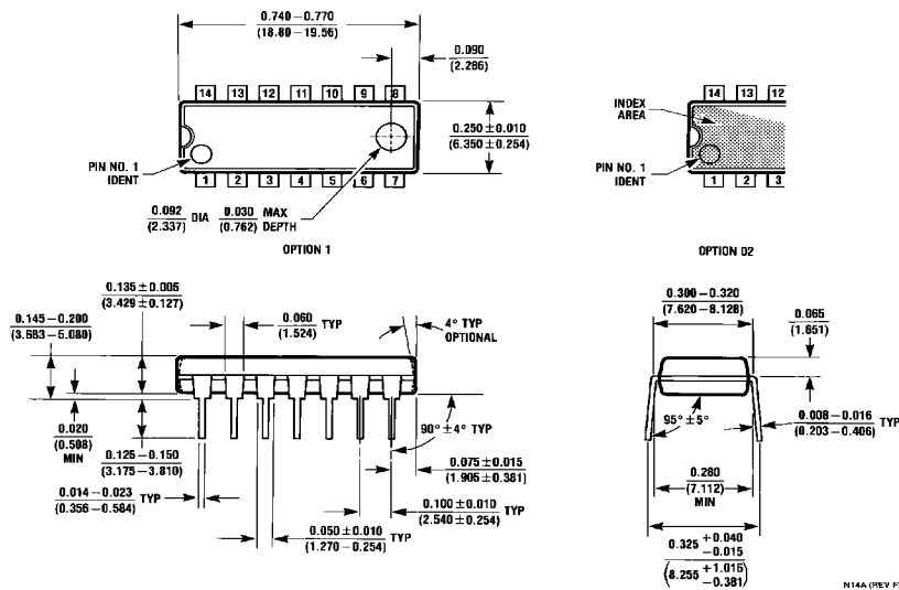
14-Lead Molded Dual-In-Line Package (N) Order Number DM7486N NS Package Number N14A
