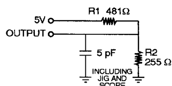
Figure 1 b Equivalent to : THEVENIN EQUIVALENT
