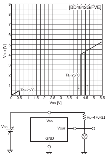
Fig.31 I/O characteristic
