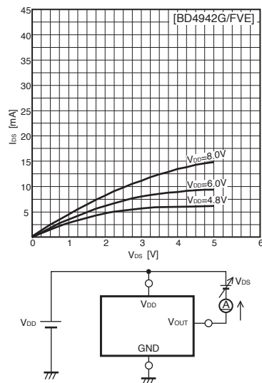
Fig.30 "H" output current
