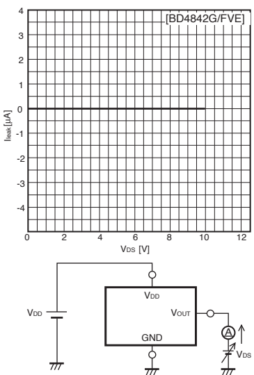
Fig.32 Output leak current
