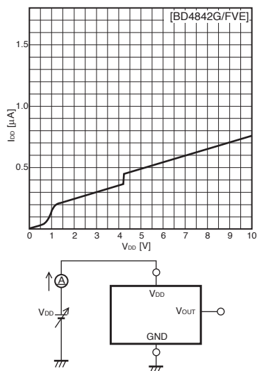
Fig.28 Circuit current
