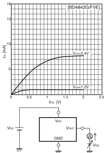
Fig.29 "L" output current
