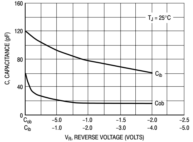
Figure 9. Capacitances
