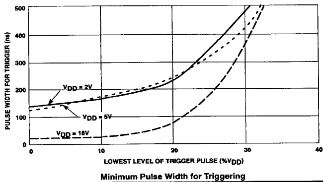
Minimum Pulse Width for Triggering
