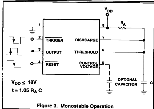
Figure 3. Monostable Operation
