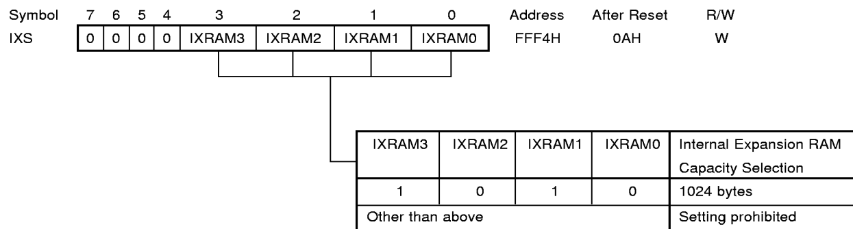
Figure 4-1. Internal Expansion RAM Size Switching Register Format
