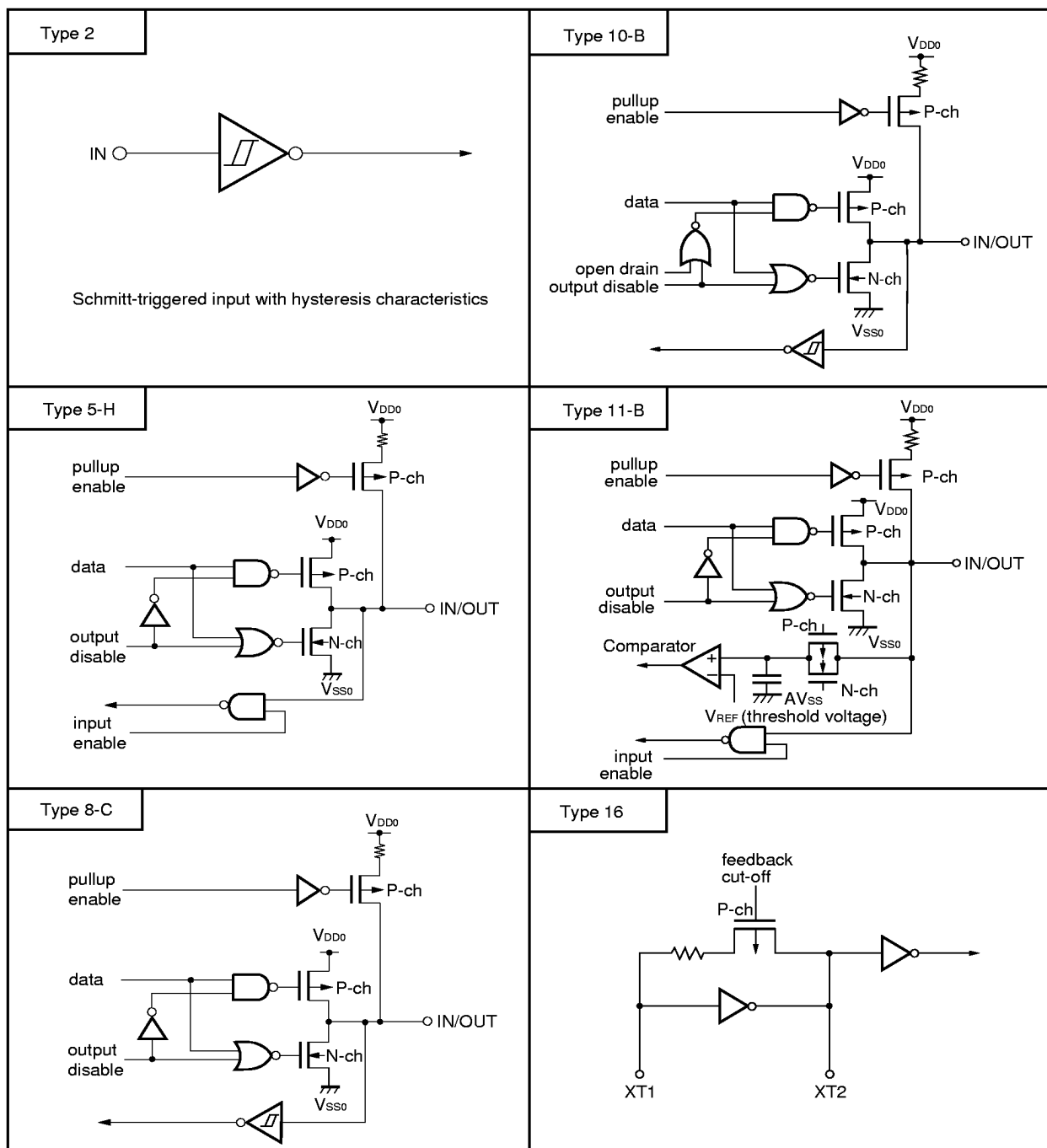
Figure 2-1. List of Pin Input/Output Circuits (1/2)
