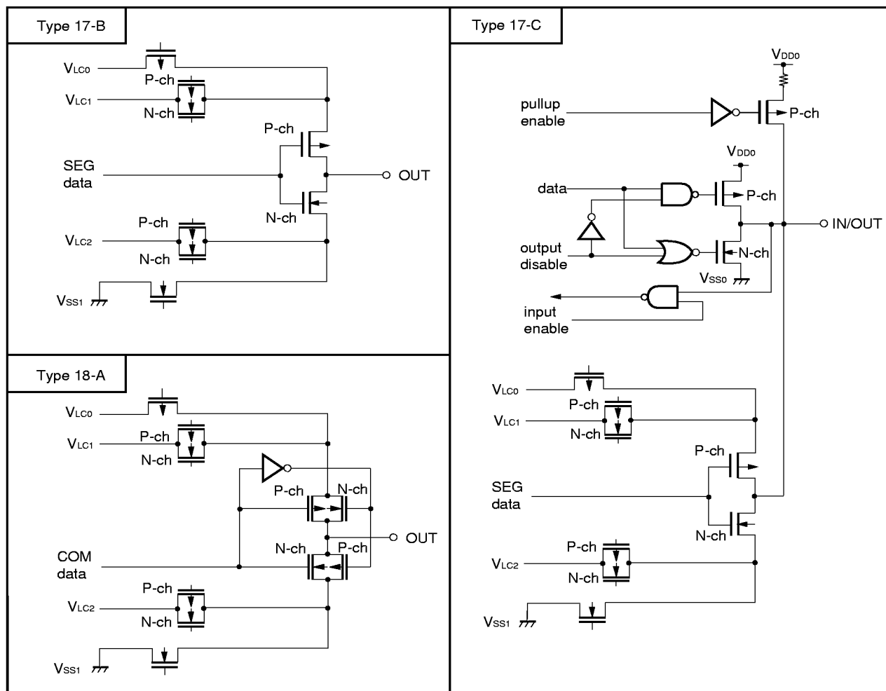
Figure 2-1. List of Pin Input/Output Circuits (2/2)
