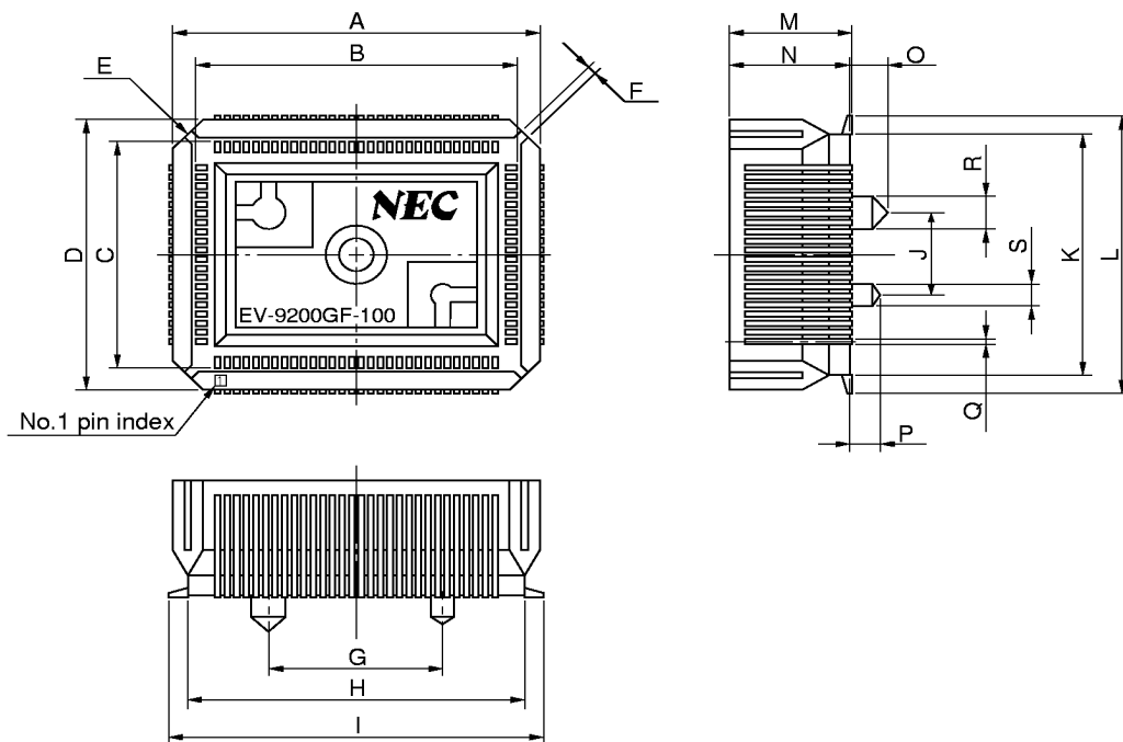
Figure A-2. Drawing of EV-9200GF-100 (for reference only)
