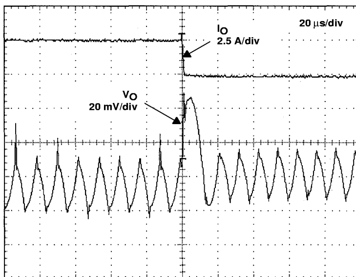
Figure 28. Falling Load Transient Response
