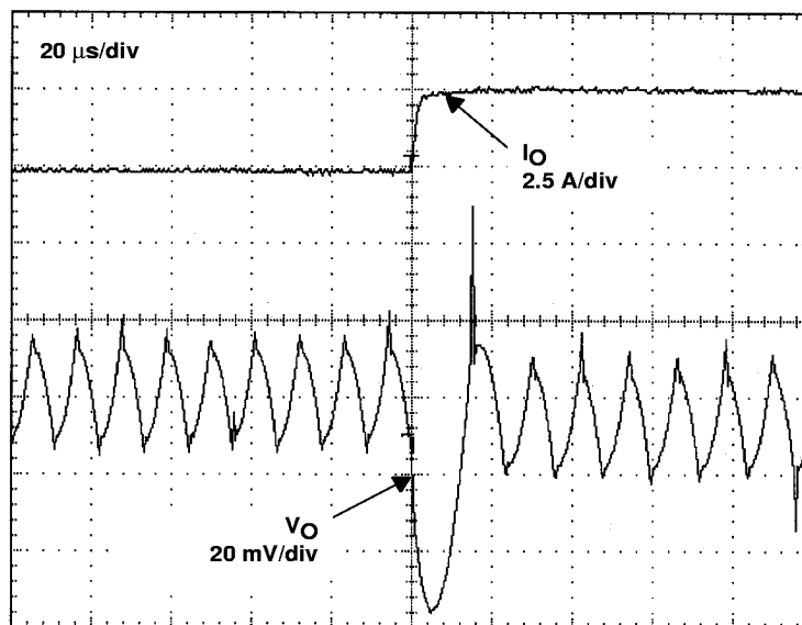
Figure 27. Rising Load Transient Response
