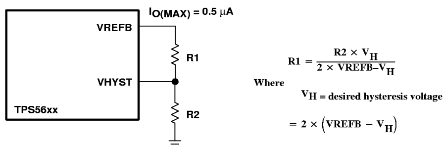
Figure 1. Setting the Hysteresis Voltage
