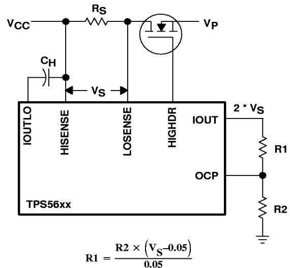
Figure 3. Precision OCP Using External Resistor
