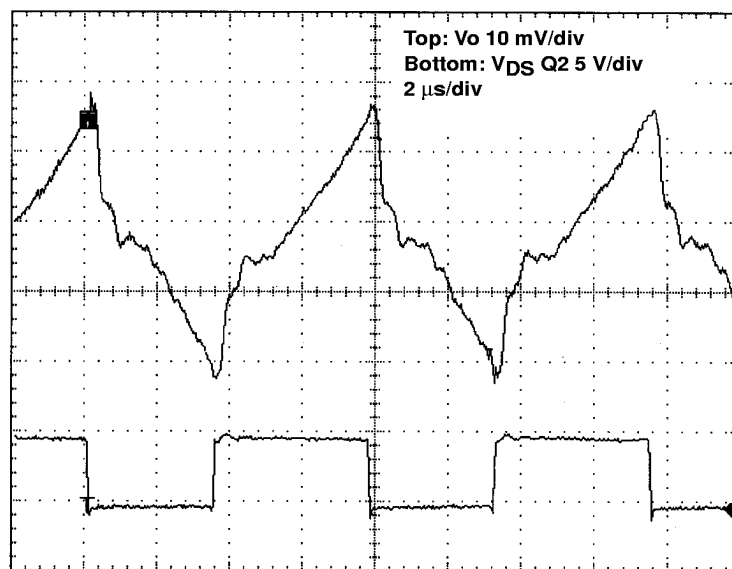
Figure 26. Output Voltage Ripple at 8 A
