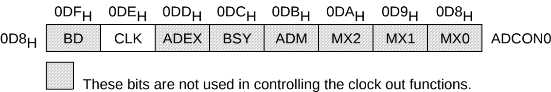
Figure 7-68 Special Function Register ADCON0 (Address 0D8H)
