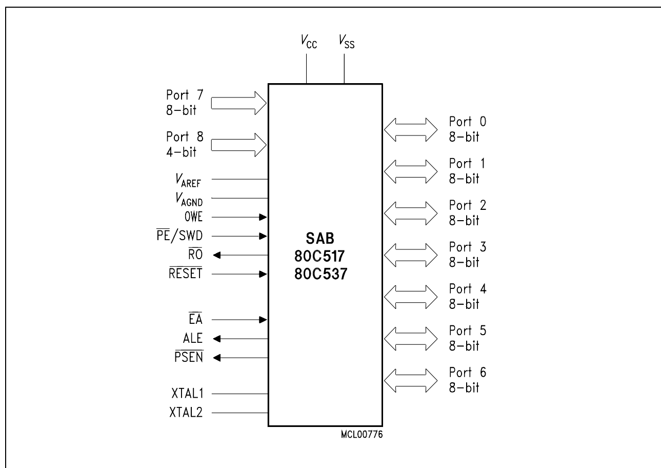
Figure 1-1 Logic Symbol
