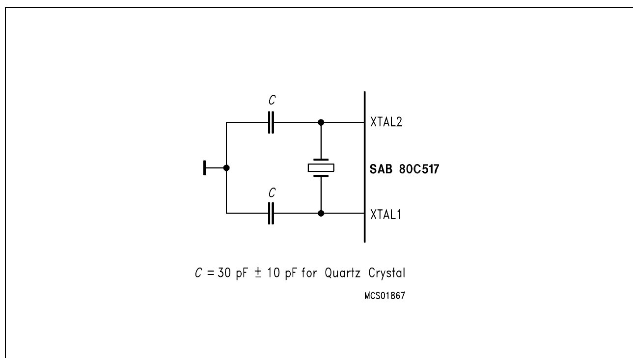
Figure 7-65 Recommended Oscillator Circuit
