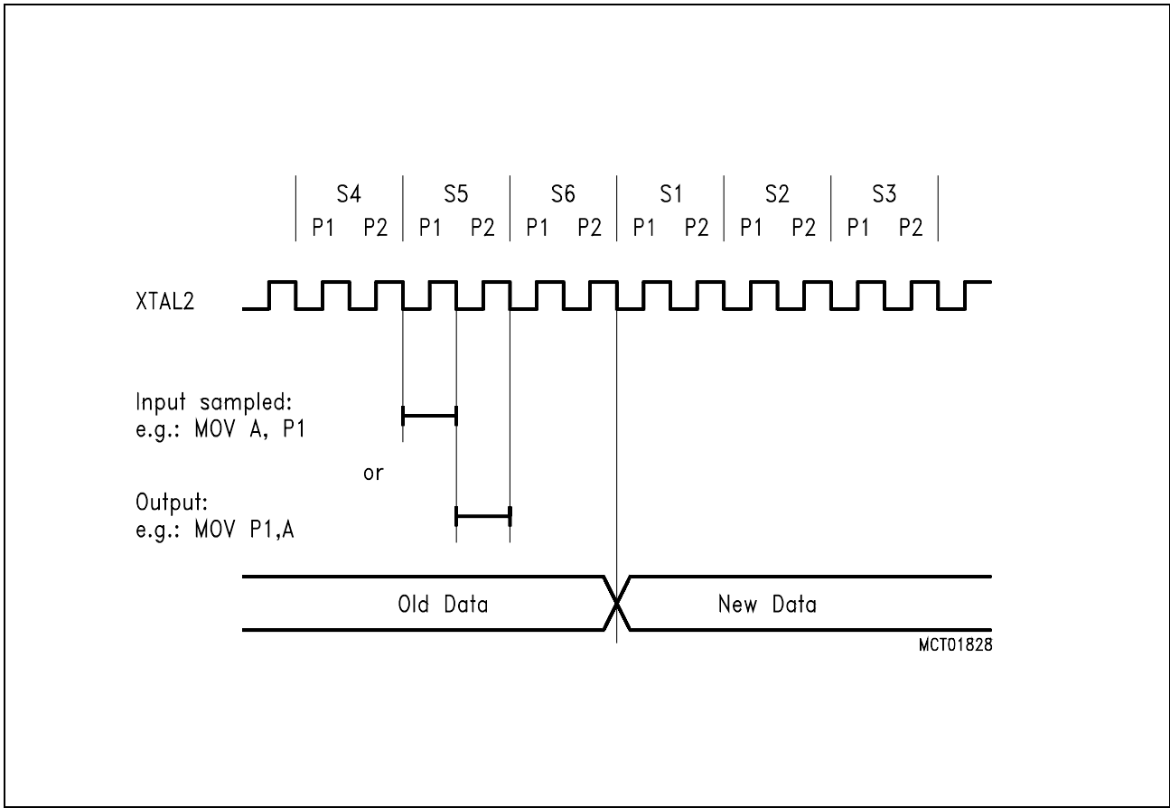
Figure 7-6 Port Timing
