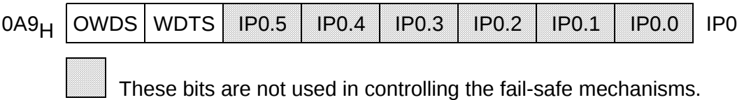
Figure 7-63 Special Function Register IP0
