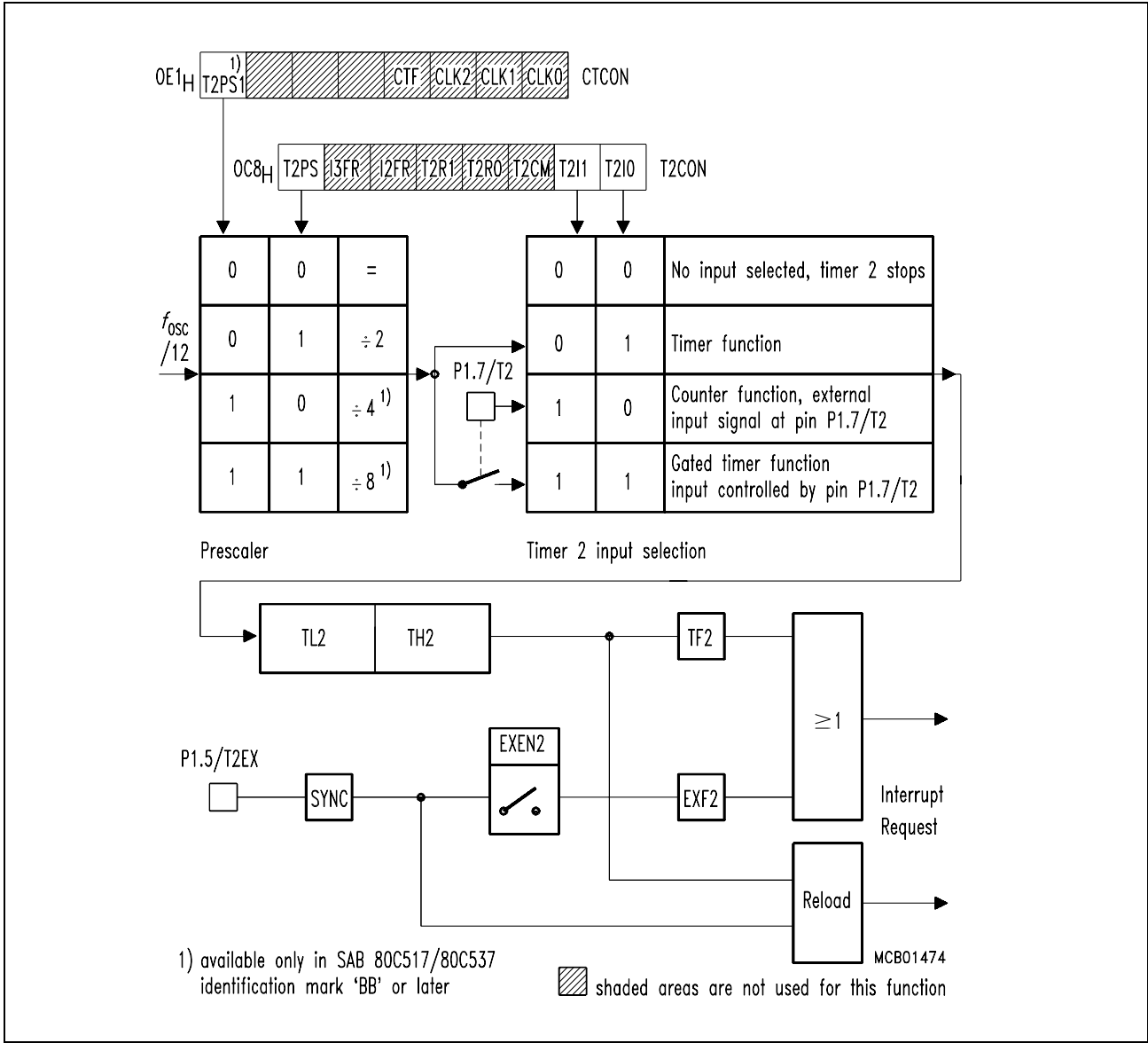
Figure 7-34 a) Block Diagram of Timer 2
