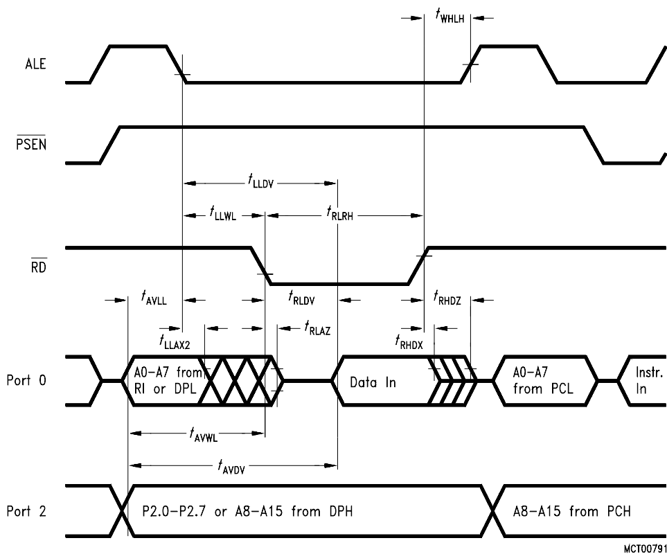
Data Memory Read Cycle
