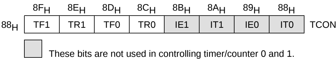
Figure 7-19 Special Function Register TCON (Address 88 H )
