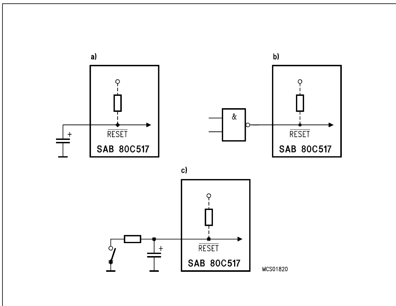
Figure 6-1 Reset Circuitries
