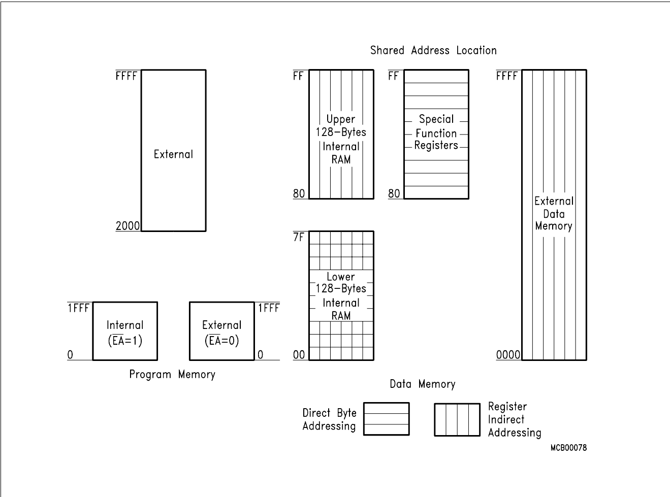
Figure 2 Memory Mapping
