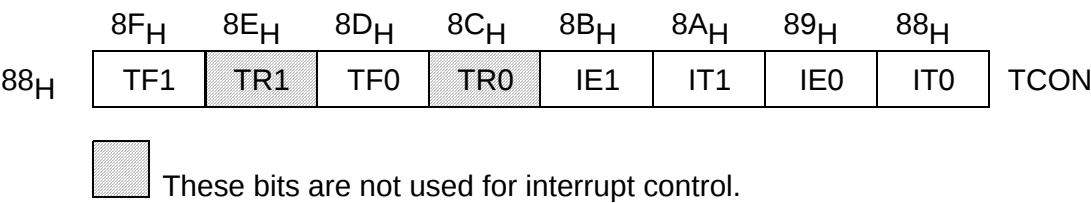
Figure 8-5 Special Function Register TCON (Address 88 H )
