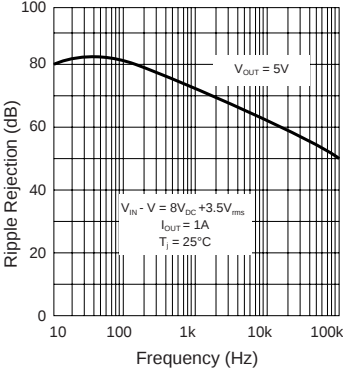
RIPPLE REJECTION
