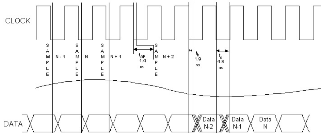
Figure 4. Timing diagram
