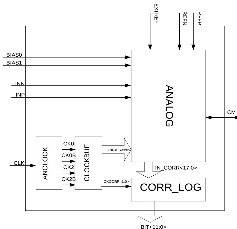
Figure 1. Block diagram nAD1260-25
