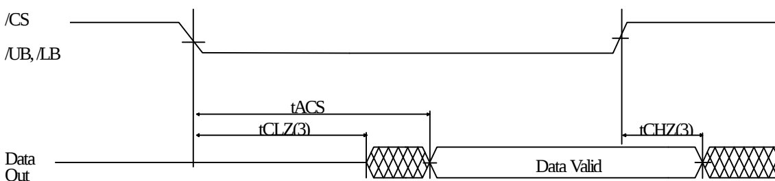
READ CYCLE 3(Note 1,2,4)
