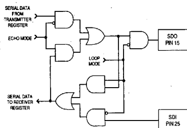
Figure 10 : LOOP and ECHO MODE FUNCTIONALITY
