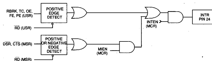
Figure 15 : INTERRUPT STRUCTURE
