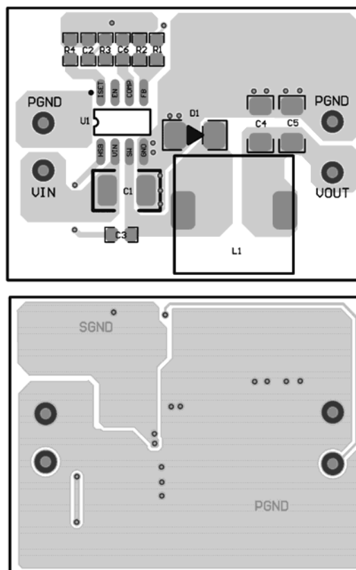
Figure 7: PCB Layout
