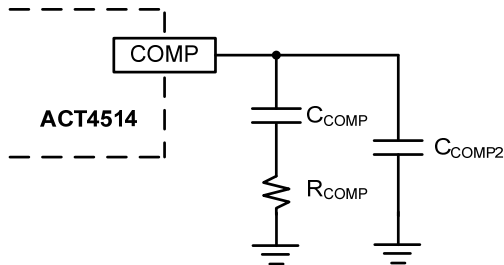
Figure 4: Stability Compensation
